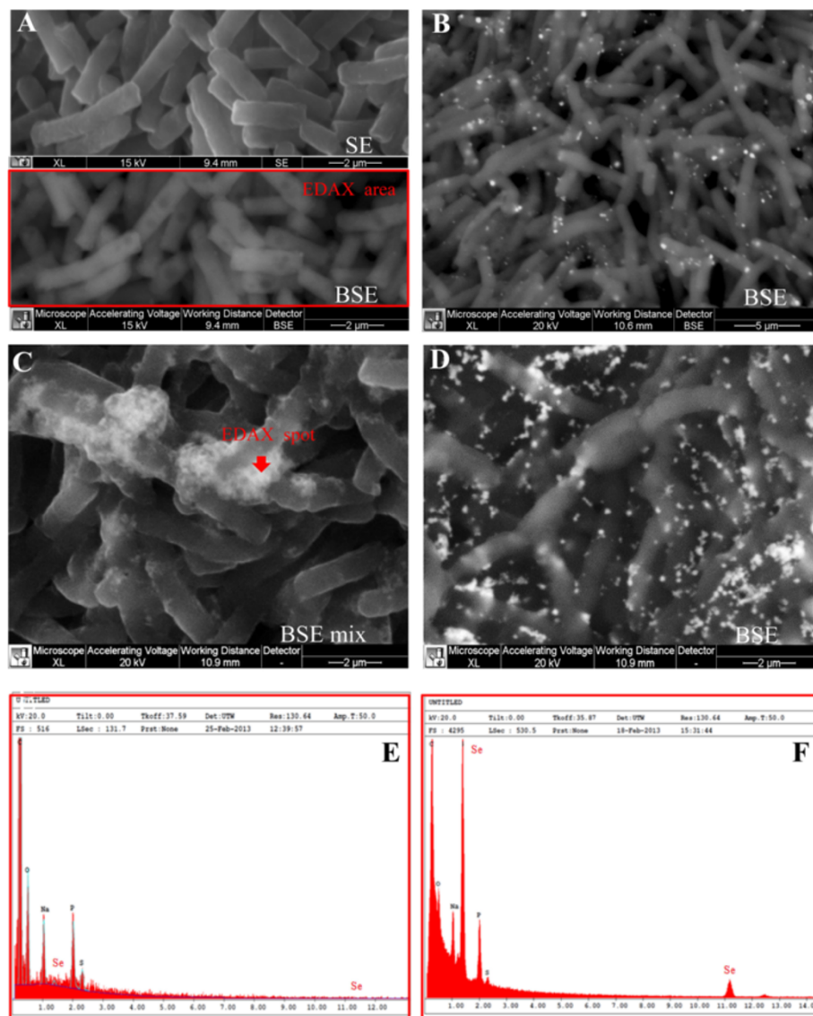
Figure 6 SEM micrographs and EDAX spectra of B. mycooides SeITE01 cultures grown in absence (A), or in presence of 2.0 mM \text{SeO}_3^{2-} , at increasing incubation times: 6 (B), 24 (C), and 48 (D) hours, in panel (E) and (F) are shown EDAX spectra corresponding to control and 24 hours SeITE01 culture, respectively. SE and BSE stand for Secondary Electrons and Back-Scattered Electrons signal, respectively.
