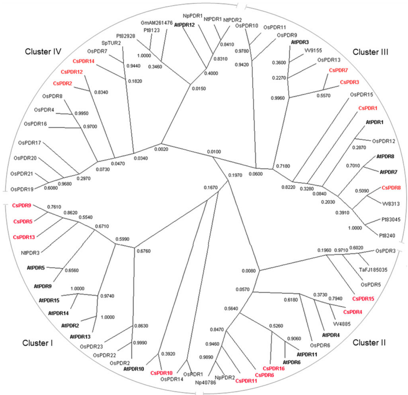
Fig. 4 Phylogenetic relationships of the 16 predicted PDR-like transporters identified in cucumber and PDR-like representatives from other plants. The unrooted tree was constructed by the MEGA5.1 software (Tamura et al. 2011) using the neighbor-joining method with 1,000 bootstrap replicate trees. The accession numbers are as follows: Arabidopsis thaliana , AtPDR1 (DAA00870), AtPDR2 (DAA00869), AtPDR3 (DAA00871), AtPDR4 (DAA00872), AtPDR5 (DAA00873), AtPDR6 (DAA00874), AtPDR7 (DAA00875), AtPDR8 (DAA00876), AtPDR9 (DAA00877), AtPDR10 (DAA00878), AtPDR11 (DAA00879), AtPDR12 (DAA00880), AtPDR13 (DAA00881), AtPDR14 (DAA00882), AtPDR15 (DAA00883); Oryza sativa , OsPDR1 (CAD59576 or Q8GU82), OsPDR2 (CAD59575 or Q8GU83), OsPDR3 (CAD59574 or Q8GU84), OsPDR4 (DAA00887), OsPDR5 (Q8GU86), OsPDR6 (Q8GU87), OsPDR7 (Q8U88 or CAD59570), OsPDR8 (Q8GU89 or CAD59569),
