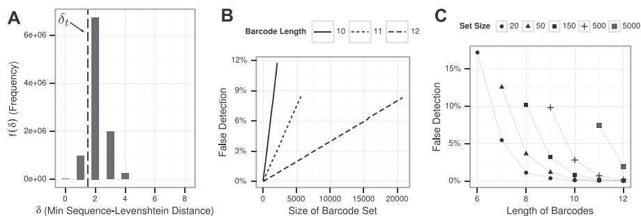
Figure 2 Similarities between 10 million random subsequences of the Mus musculus DNA database and barcode sets of different sizes and barcode lengths. (A) Distribution of minimal distances f(\delta) between 150 [8,3] barcodes and subsequences. The separation by a naive threshold \delta_t = 1 is illustrated by a vertical dashed line. (B) Falsely detected subsequences as proportion of all tested subsequences based on a threshold of \delta_t = d_{SL}(\text{barcode}, \text{subsequence}) \leq 1 for different sizes of the barcode set and barcodes of length 10 nt, 11 nt and 12 nt (C) Falsely detected subsequences as proportion of all tested subsequences based on a threshold of \delta_t = d_{SL}(\text{barcode}, \text{subsequence}) \leq 1 for different barcode lengths.
