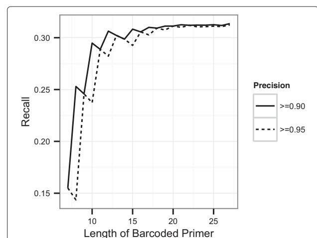
Figure 6 Sensitivity of detecting reads with barcodes depending on length of barcoded reference primer. Sensitivity was calculated for two different precision levels over barcoded reference primer lengths from 7 nt (just the reference barcode) to 27 nt (7 nt reference barcode plus 20 nt of reference primer appended). The staircase effect occurs due to discrete threshold steps and fixed precision levels.
