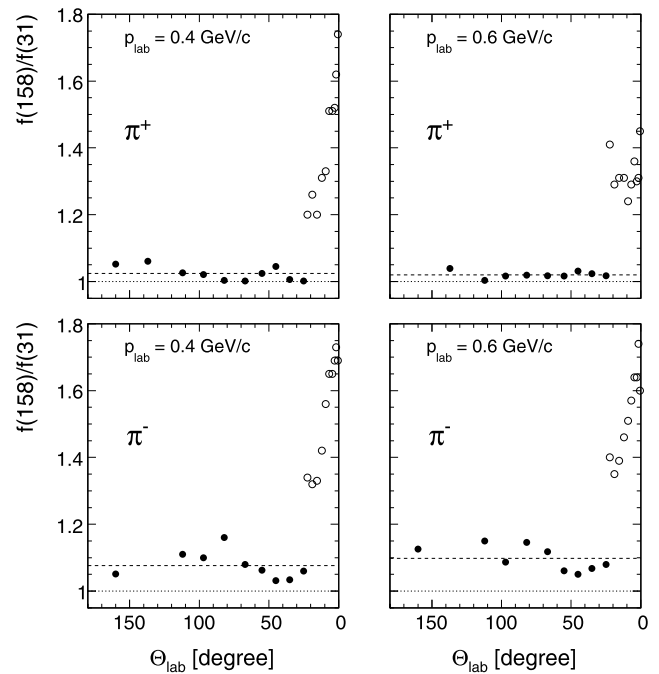
Fig. 38 Ratio of invariant pion cross sections at 158/400 and 31 GeV/c as a function of \Theta_{lab} for p_{lab} = 0.4 and 0.6 \text{ GeV}/c . The full circles correspond to the global data interpolation, the open circles to the direct ratio [13]/[15]. The broken lines give the mean ratio over the complete range of the global data interpolation
