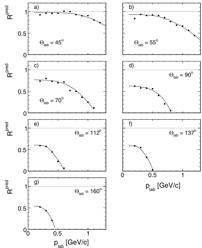
Fig. 41 R^{\text{pred}}(p_{\text{lab}}, \Theta_{\text{lab}}) as a function of p_{\text{lab}} for the angles of 45, 55, 70, 90, 112, 137 and 160 degrees. The full lines are local interpolations
