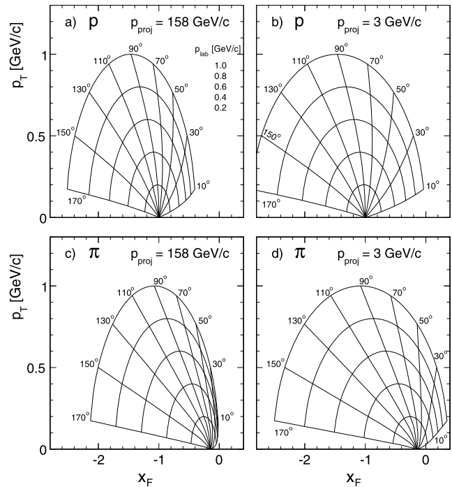
Fig. 1 Lines of constant p_{lab} and \Theta_{lab} in the cms frame spanned by Feynman x_F and p_T for protons and pions at two different projectile momenta, (a) protons at 158 GeV/c, (b) protons at 3 GeV/c, (c) pions at 158 GeV/c and (d) pions at 3 GeV/c
