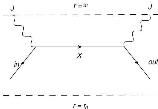
Figure 1. Five-dimensional tree-level Witten's diagram which is the holographic dual version of the forward Compton scattering of a charged lepton by a hadron in four-dimensions. This diagram is made of five-dimensional fields obtained from dimensional reduction of ten-dimensional supergravity on a compact Einstein manifold. The dual field of the hadron is indicated with a solid line. The hadron can be a scalar, a N_f = 1 vector meson, or a N_f > 1 vector meson. Wavy lines indicate the dual field corresponding to a virtual photon exchanged from the lepton (not drawn in this diagram) and the hadron. This field (wavy line) is a fluctuation induced by the insertion of the global symmetry current operator at the boundary theory. This Witten's diagram gives the leading contribution to the 1/N expansion. Notice that r \rightarrow \infty corresponds to the boundary where the four-dimensional gauge theory is defined and where current operators J are inserted.
