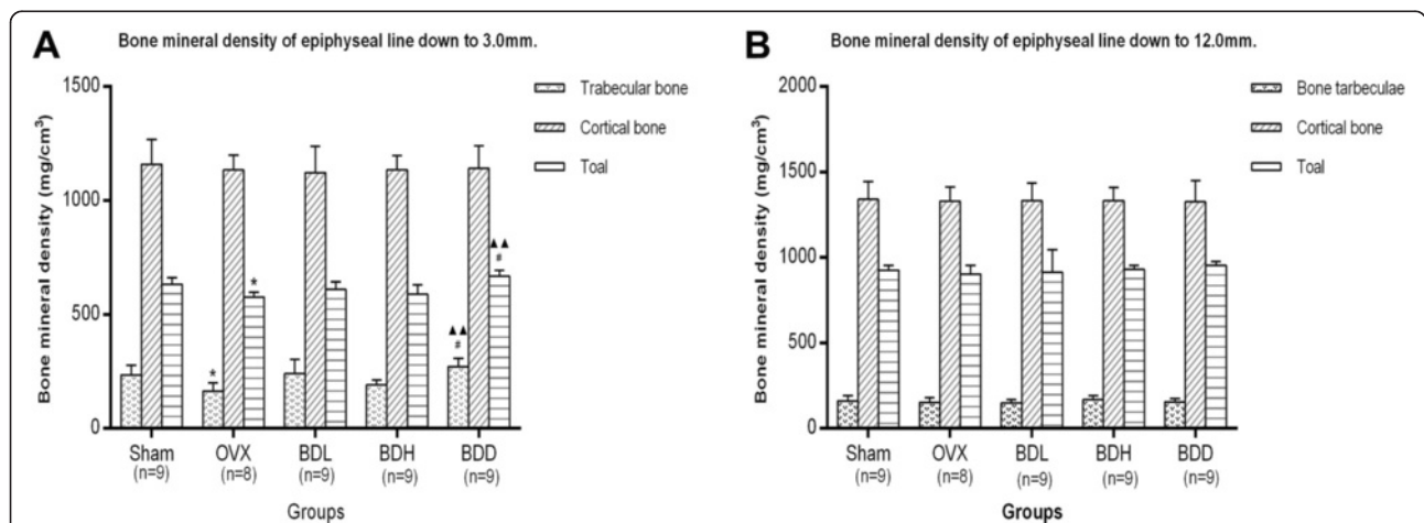
Fig. 3 Effects on the BMD. a showed that the density of trabecular bone and total bone density were significantly improved by Qing E formula Plus Danshen at epiphyseal line down to 3.0 mm; b showed that there was no apparent difference shown at the epiphyseal line down to 12.0 mm. *P < 0.05 vs. Sham group; ▲▲P < 0.01 vs. OVX group; #P < 0.05 vs. BDH group
