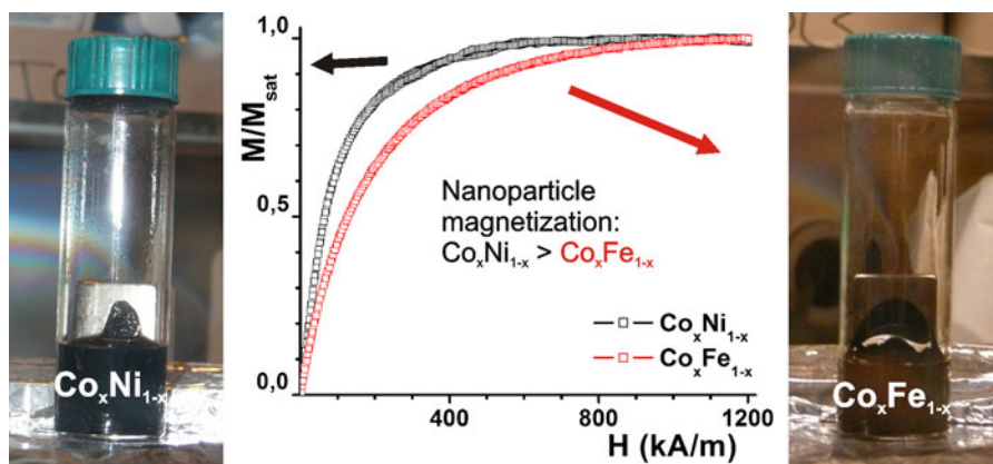
Fig. 5 Pictures of \text{Co}_x\text{Ni}_{1-x} (left) and \text{Co}_x\text{Fe}_{1-x} (right) dispersions in dioctyl ether when held against a 1.3 T magnet. Typical, normalized magnetization curves of \text{Co}_x\text{Ni}_{1-x} (black,
