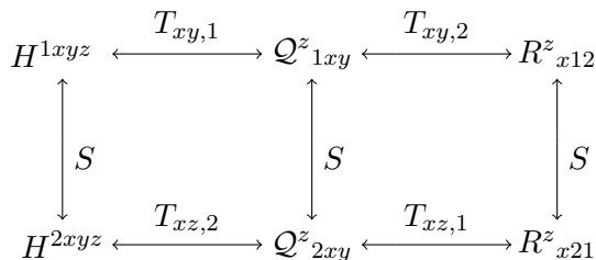
Figure 1. Duality relations involving 3-form, Q- and new R-flux in IIB.
