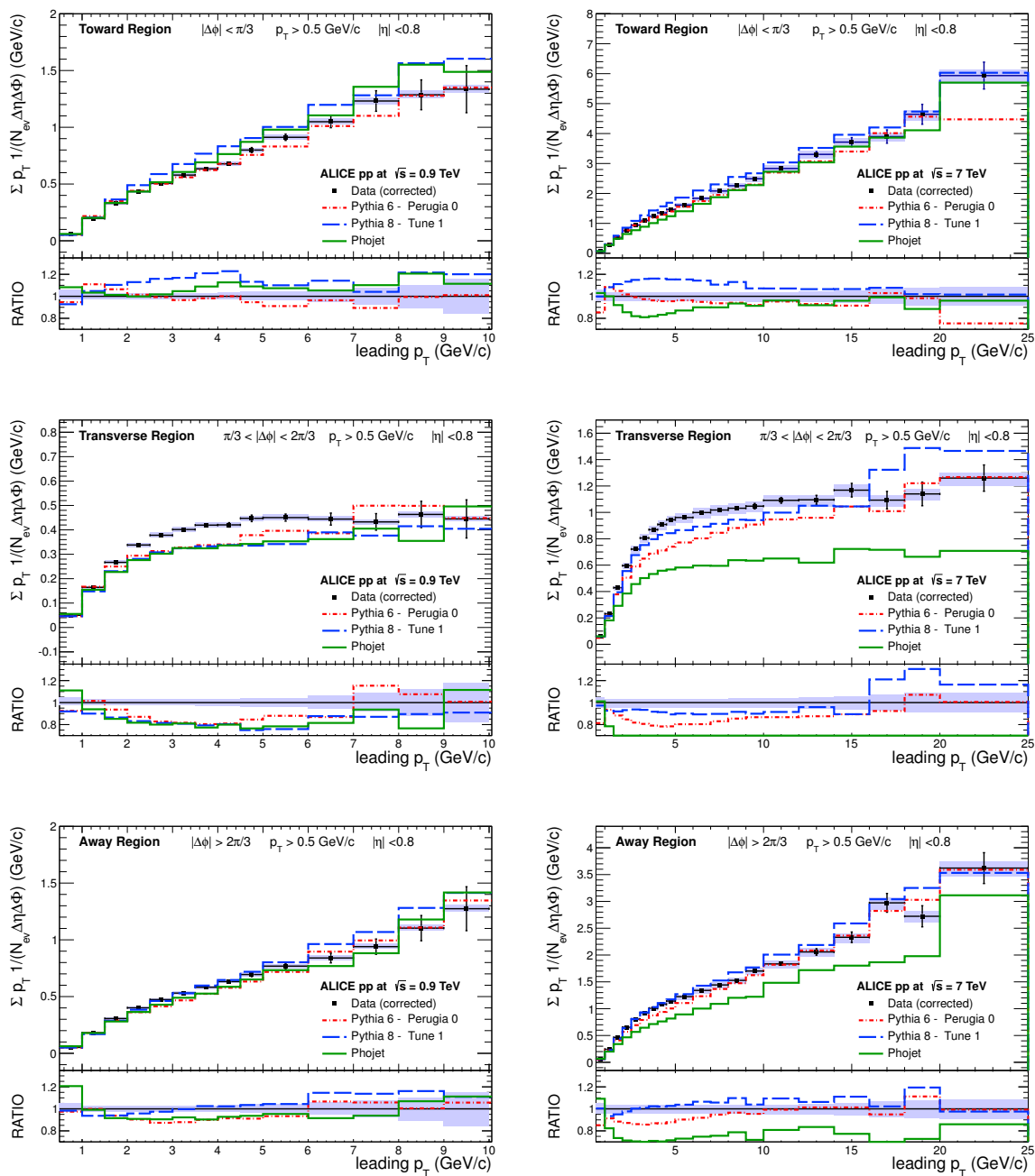
Figure 10. Summed p_T in Toward (top), Transverse (middle) and Away (bottom) regions at \sqrt{s} = 0.9 TeV (left) and \sqrt{s} = 7 TeV (right). Right and left vertical scales differ by a factor 4 (2) in the top (middle and bottom) panel. Shaded area in upper plots: systematic uncertainties. Shaded areas in bottom plots: sum in quadrature of statistical and systematic uncertainties. Horizontal error bars: bin width.
