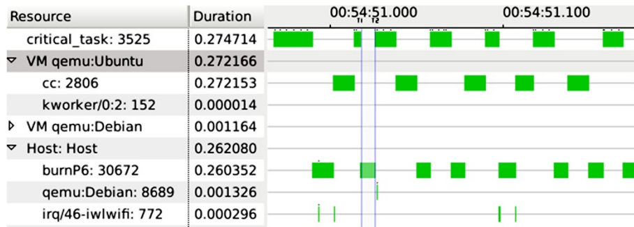
Figure 14 Execution flow recovery of problematic critical_task.
