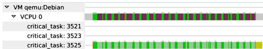
Figure 13 Magnified view of the execution of critical_task 3525.
