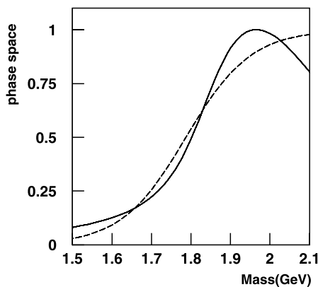
Fig. 3 f_2(1270)\eta phase space (full curve) and an approximation with a Fermi function (dashed)
