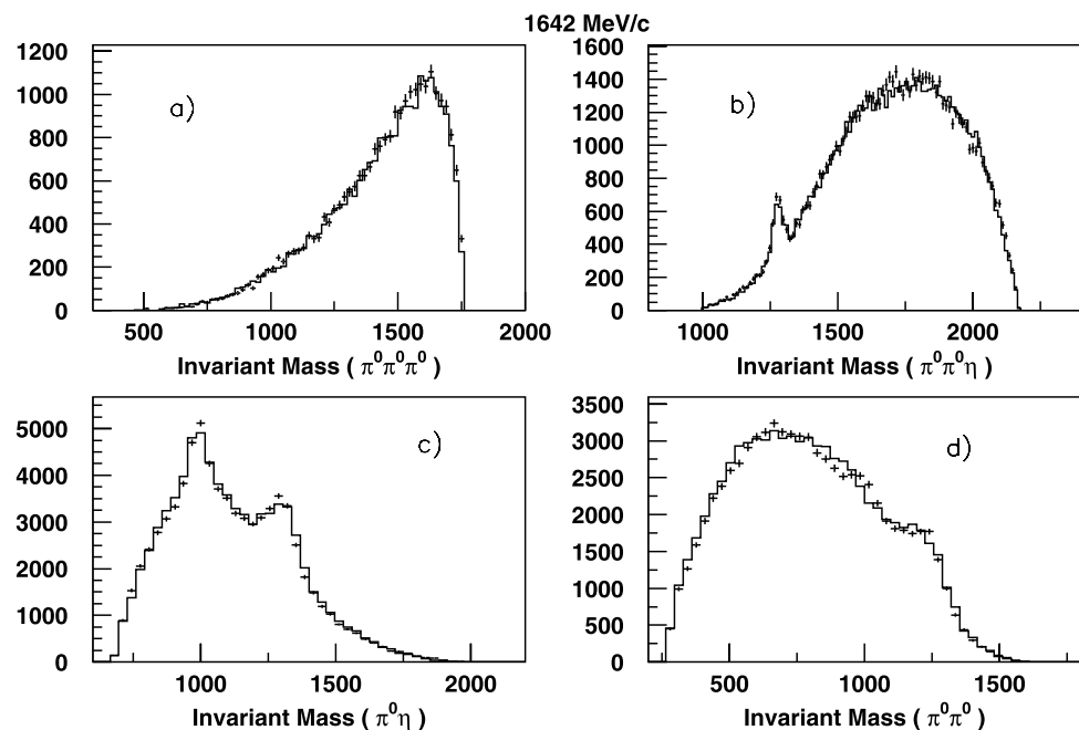
Fig. 4 Mass spectra for (a) 3\pi , (b) \eta\pi\pi , (c) \eta\pi and (d) \pi\pi at a beam momentum of 1642 MeV/c. Histograms show fits to data
