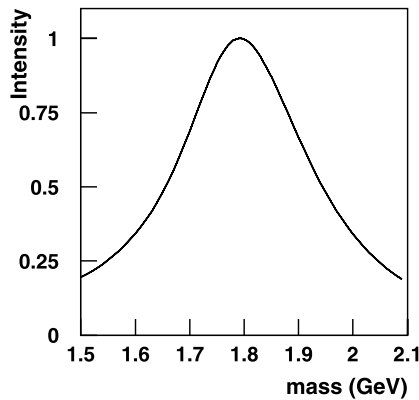
Fig. 10 The line-shape of \eta_2(1870) from the combined fit to CBAR and WA102 data
