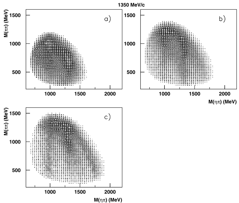
Fig. 1 Scatter plots of M(\pi\pi) vs. M(\eta\pi) for three ranges of M(\eta\pi\pi) : (a) 1560–1750 MeV, centred on \eta_2(1645) , (b) 1775–1945 MeV over \eta_2(1870) and (c) 1945–2115 MeV, centred on \eta_2(2030) . The beam momentum is 1350 MeV/c
