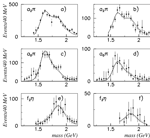
Fig. 9 Fits to WA102 data for central production of a_2\pi , a_0\pi and f_2(1270)\eta with J^{PC} = 2^{-+} . The first column shows data for \eta \rightarrow \gamma\gamma and the second data for \eta \rightarrow \pi^+\pi^-\pi^0 . Full curves are fits without \eta_2(2030) and dashed curves with it
