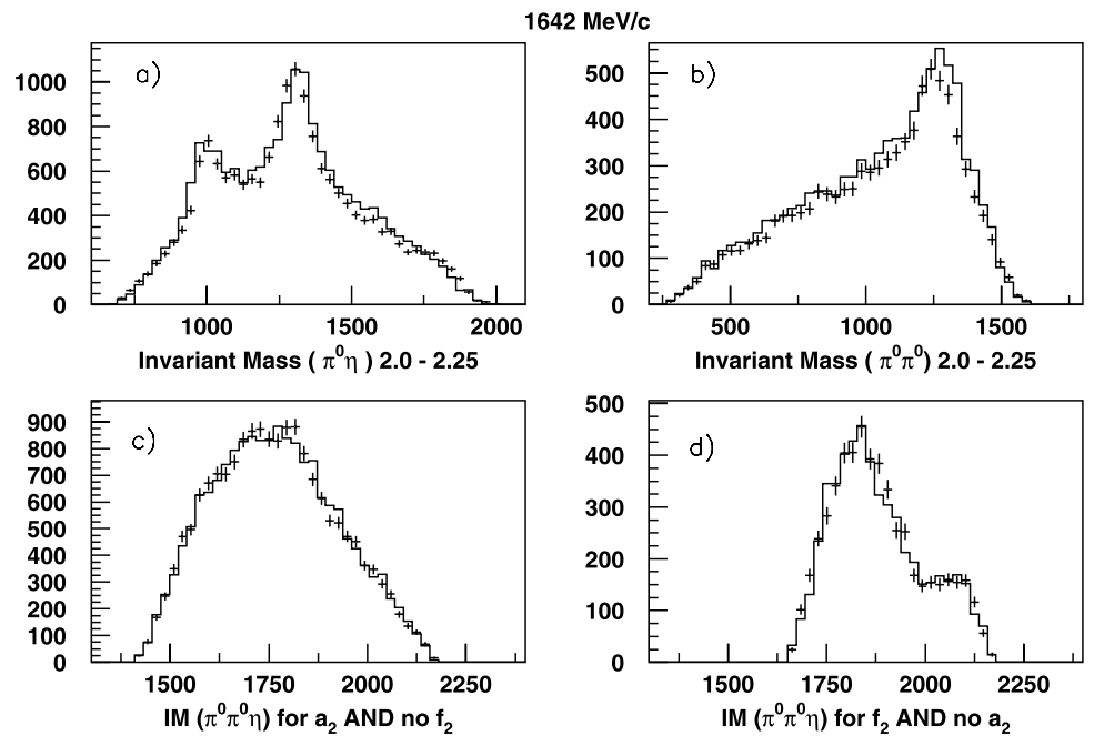
Fig. 6 Mass spectra at 1642 MeV/c for (a) and (b) \pi^0\eta and \pi^0\pi^0 in the M(\pi\pi\eta) mass range 2.0–2.25 GeV; (c) the \pi\pi\eta mass spectrum selecting a_2 and vetoing f_2(1270) ; (d) the converse selection. Histograms show fits to data
