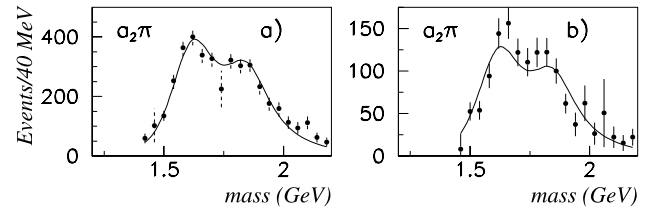
Fig. 11 Fits to WA102 data with \eta_2(1870) \rightarrow a_2\pi replaced by f_2(1910) \rightarrow a_2\pi : (a) \eta \rightarrow \gamma\gamma , (b) \eta \rightarrow \pi^+\pi^-\pi^0
