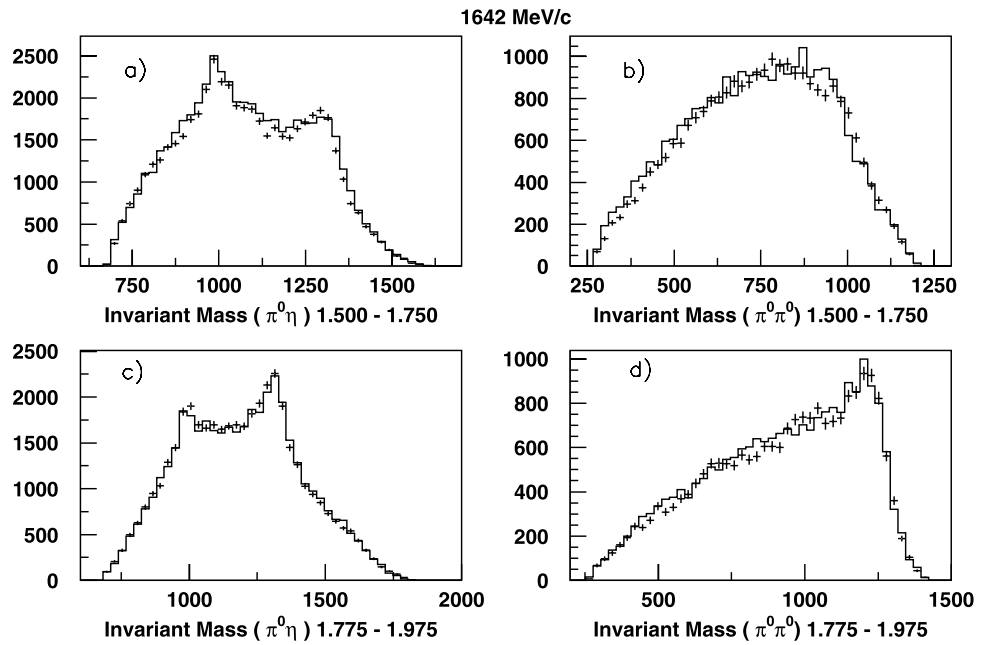
Fig. 5 Mass spectra at 1642 MeV/c for (a) and (c) \pi^0\eta in two ranges of M(\pi\pi\eta) ; (b) and (d) \pi^0\pi^0 . Histograms show fits to data
