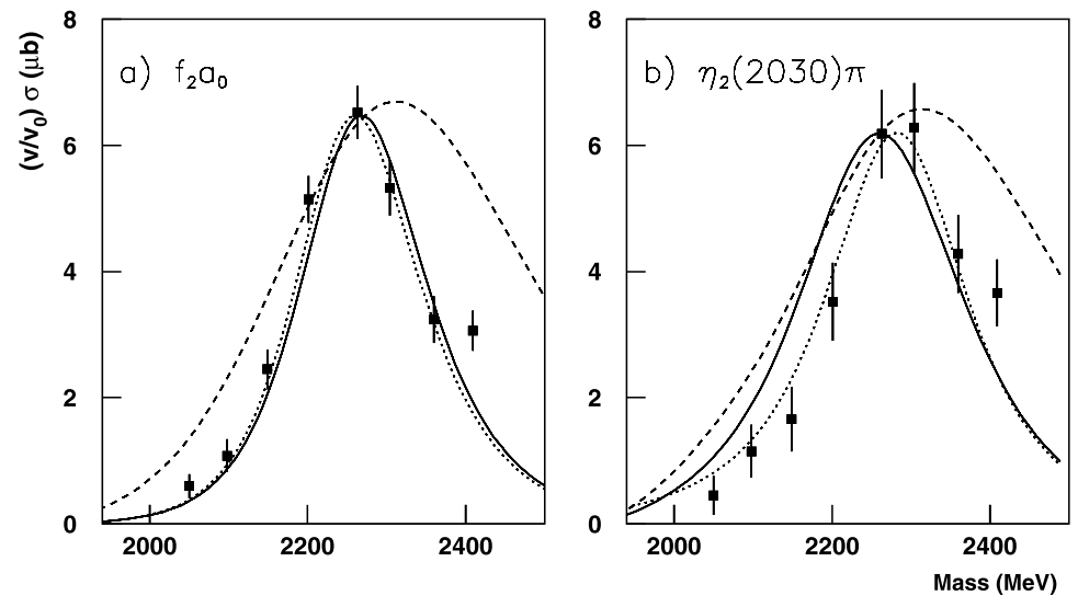
Fig. 8 Production of (a) f_2(1270)a_0 compared to phase space for S-wave production (dashed curve), a fit to f_2(2255) (full curve) and a fit with parameters of this state optimised (dotted curve); (b) \eta_2(2030)\pi compared to phase space for P-state production (dashed curve), a fit using the line-shape of \pi_2(2245) (full curve) and a fit with parameters of this state optimised (dotted)
