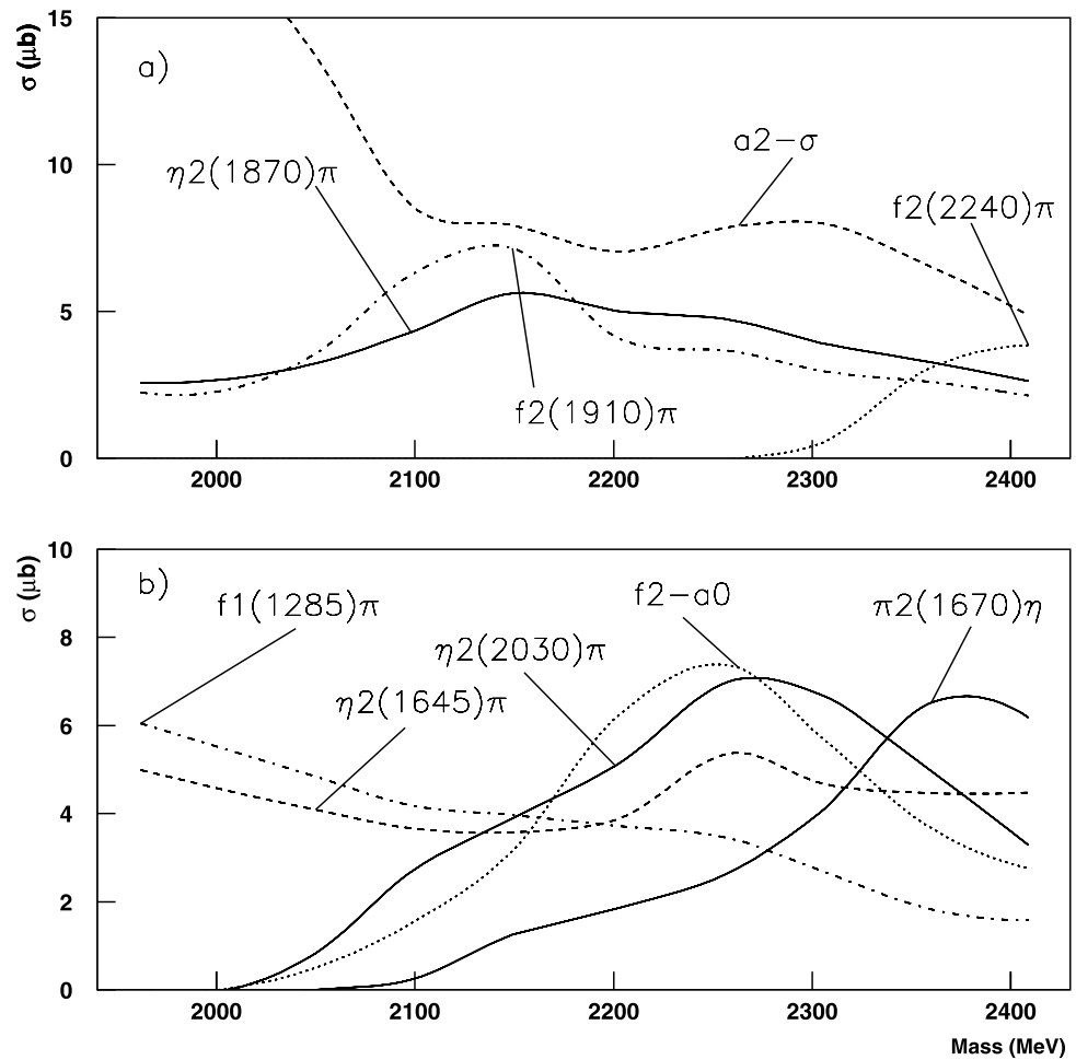
Fig. 7 Cross sections for each final state. Smooth curves are drawn through cross sections for each channel
