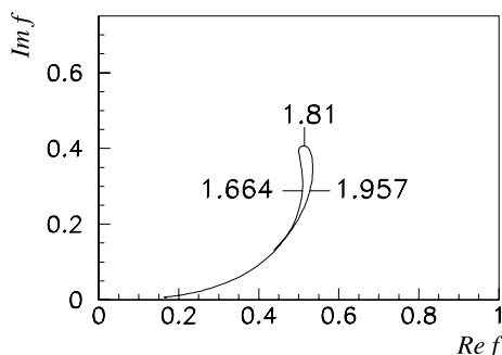
Fig. 12 The Argand diagram for a fit to WA102 data using (26)
