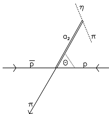
Fig. 2 A sketch of \bar{p}p \rightarrow a_2(1320) \rightarrow \eta\pi
