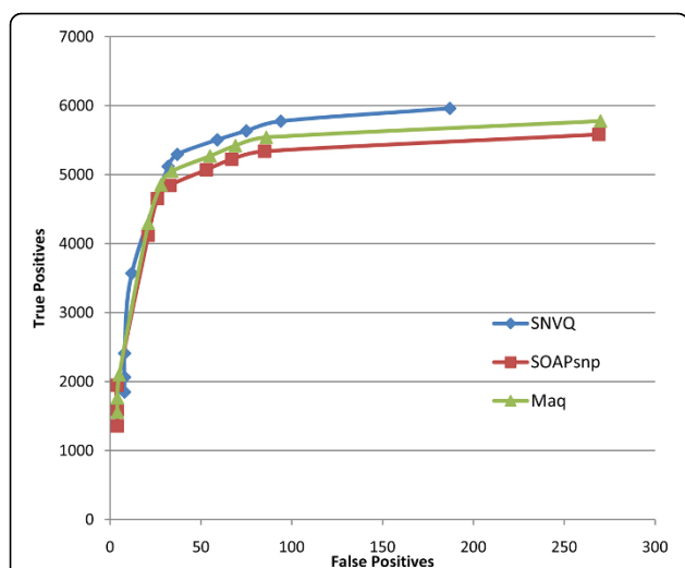
Figure 8 Genotyping accuracy of SNVQ, SOAPsnp, and Maq on RNA-Seq reads pooled from Hapmap individuals NA12878, NA18498, and NA18517.
