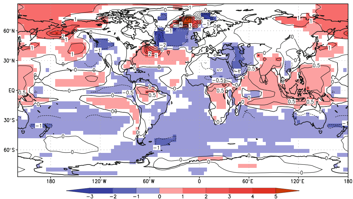
Fig. 7 Differences in December–March temperature between the IOWP25 and CNTL simulations ( ^{\circ}\text{C} , color; values are SST over ocean and 2-m temperature over land). Colors are shown only where temperature differences exceed the 95% confidence level ( t test).
