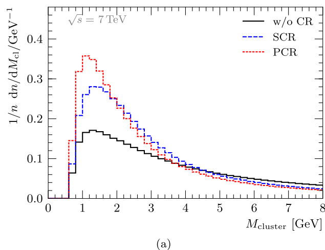
Fig. 6 Invariant mass of primary clusters in soft inclusive LHC events at 7 TeV. The histograms are normalized to unity, where also invisible bins are taken into account. The histograms in (b) differ from the ones in (a) only in their binning
