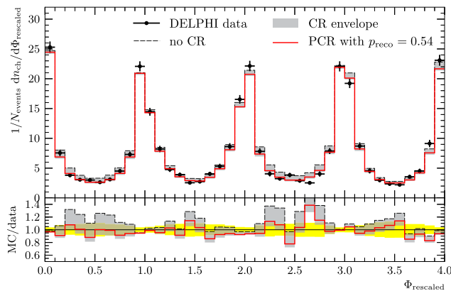
Fig. 11 Charged-particle flow in hadronic WW events at LEP with \sqrt{s} = 189 GeV. The grey band indicates the range which is covered by varying the colour reconnection strength p_{reco} in the PCR model. The definition of the rescaled angle, \Phi_{rescaled} , along with a detailed description of the analysis can be found in Ref. [52]
