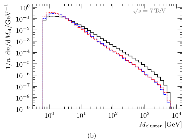
Fig. 6 Invariant mass of primary clusters in soft inclusive LHC events at 7 TeV. The histograms are normalized to unity, where also invisible bins are taken into account. The histograms in (b) differ from the ones in (a) only in their binning
