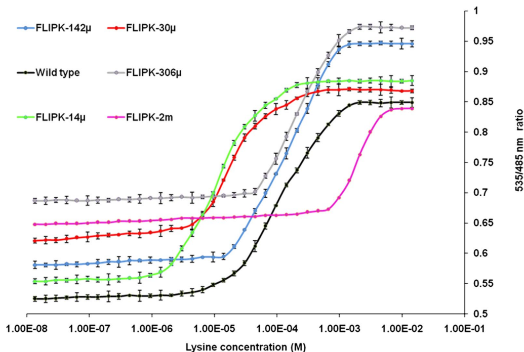
Fig. 6 In vitro ligand dependent FRET ratio change of FLIPK in the presence of L-lysine. Affinity mutants Y14A, R77L, F52A, D161I and S72A were developed. Mutations at position 14 tyrosine substituted by alanine (Y14A), arginine 77 to leucine (R77L), phenylalanine 52 to alanine (F52A), and aspartic acid 161 to isoleucine (D161I) and serine at 72 position by alanine (S72A). Concentration of sensor protein was 0.24 mg/ml. Values are means of three independent replications. Vertical bars indicate standard error
