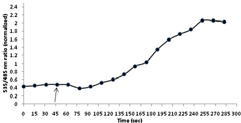
Fig. 9 Lysine concentration change in the cytosol of yeast. S. cerevisiae /URA3 strain BY4742 expressing the sensor FLIPK. The graph indicates the emission intensity ratio (535/485 nm ratio) for a single yeast cell. Addition of 100 mM lysine (shown by arrow) increased the ratio by 2.0
