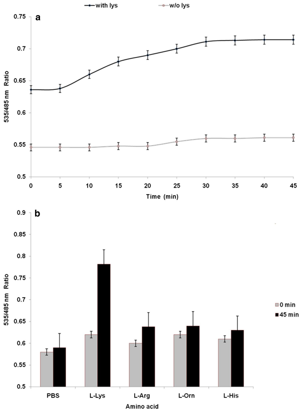
Fig. 7 In vivo analysis of the FLIPK (WT) nanosensor. a FRET ratio change in response to the 10 mM lysine (black circles) and without lysine (grey circles) in 20 mM PBS buffer. b FRET (535/485 nm) ratio of the bacterial cell suspension before and after incubation with various amino acids for 45 min
