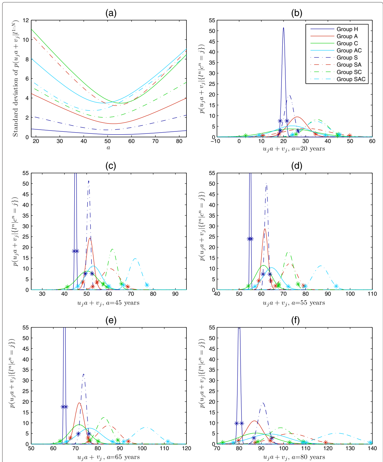
Figure 6 Posterior distributions p(u_j a + v_j | \{l^m | c^n = j\}) . (a) : Standard deviations of the posterior distribution p(u_j a + v_j | \{l^m | c^n = j\}) . (b-f) : Posterior distributions p(u_j a + v_j | \{l^m | c^n = j\}) for ages a = 20, 45, 55, 65 and 80 years. The length between two starts equals 2 \times 1.96 times the standard deviation. The legend in (b) is valid for all plots.
