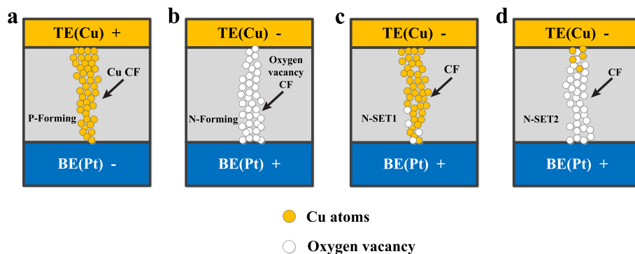
Fig. 6 Schematic illustration of the underlying working mechanism of the Cu/ZrO 2 /Pt device. a The CF illustration after P-Forming process. A Cu CF is formed to bridge the two electrodes. b The CF illustration after N-Forming process. An oxygen vacancy CF is formed to bridge the two electrodes. c The CF illustration after N-SET1 behavior. The main ingredient of the CF is Cu atoms. d The CF illustration after N-SET2 behavior. The main ingredient of the CF is oxygen vacancy
