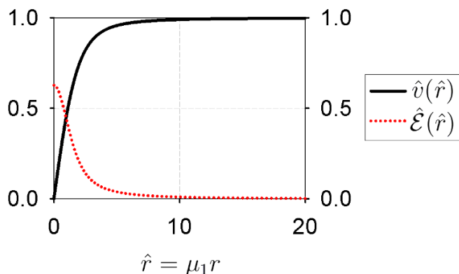
Figure 12. Plots of \hat{v}(\hat{r}) and the dimensionless energy density \hat{\mathcal{E}}(\hat{r}) for the \text{SO}(3)_{\text{HF}} invariant potential. The cut off radius for this plot is R = 20 .
