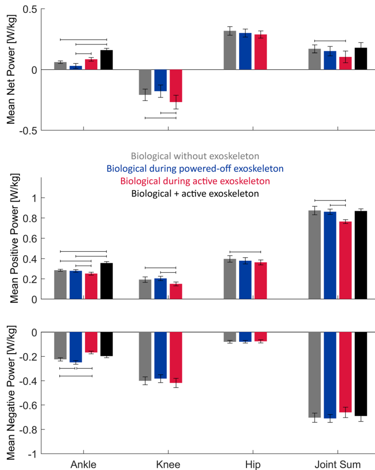
Fig. 3 Exoskeletal effects on mean joint powers. The mean net powers, mean positive powers, and mean negative powers of the biological ankle, knee, hip and sum of all three joints are shown while wearing no exoskeleton ( grey ), the powered-off exoskeleton ( blue ), and the active exoskeleton ( red ). The black bars also include the mechanical exoskeletal power. Vertical error bars represent the standard error means, and horizontal brackets denote conditions that are significantly different ( p < 0.05 )
