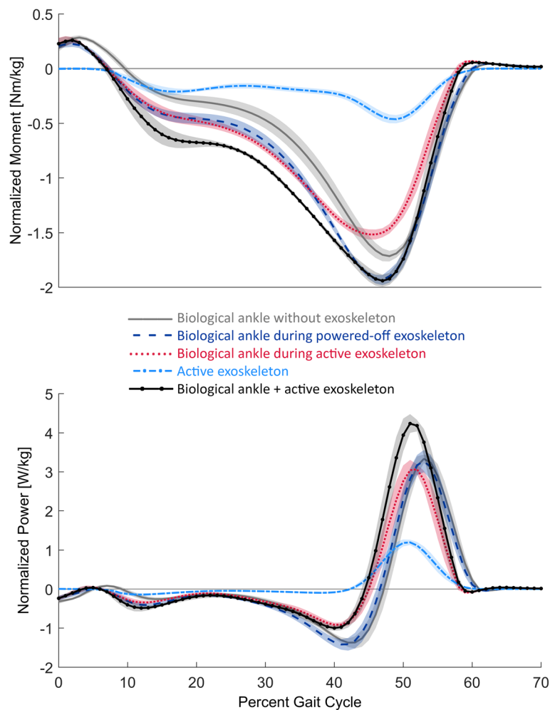
Fig. 5 Ankle moment and power profiles. The ankle moment profiles during the first 70 % of the gait cycle are depicted on the top graph, and the ankle power profiles are depicted on the bottom. Positive moment values denote ankle dorsiflexion. The figure compares the biological ankle during the no exoskeleton condition ( grey solid line ), the powered-off exoskeleton condition ( dark blue dashes ), and the active exoskeleton condition ( red dots ). The exoskeleton moment and power during the active condition are shown with light blue dashes and dots. The sum of the biological ankle and exoskeleton during the active condition are shown with a solid black line with dots. The standard error means are shown with light shading of the same color
