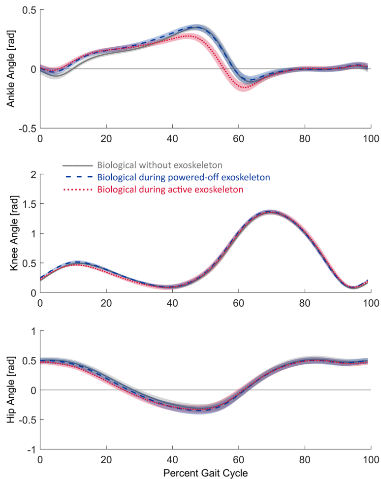
Fig. 4 Joint angle profiles. The angle trajectories of the ankle, knee and hip are shown over a gait cycle that begins and ends with heel strike of the same leg. Increasing angles represent dorsiflexion at the ankle, flexion at the knee, and flexion at the hip. The trajectories are intersubject means. The grey solid lines represent the no exoskeleton condition; dark blue dashes represent the powered-off exoskeleton condition, and the red dots represent the active exoskeleton condition. The standard error means are shown with light shading of the same color
