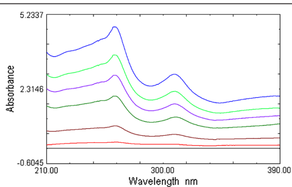
Figure 7 Ratio spectra of CEF (1 to 15 µg/mL) using 8 µg/mL solution of MOX as divisor.
