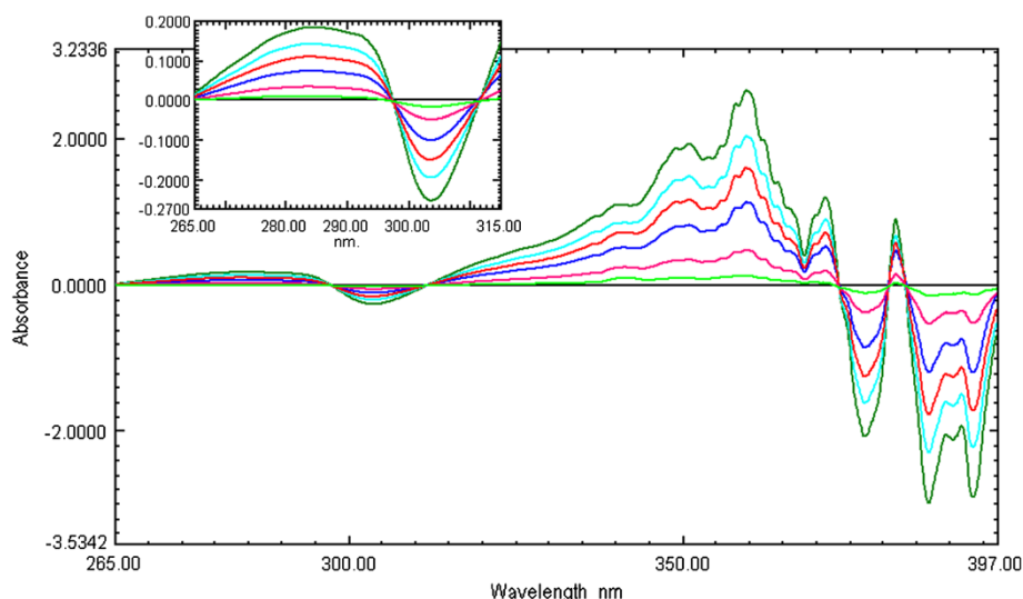
Figure 6 First derivative Ratio spectra of MOX (1 to 15 µg/mL), inside enlarged portion of spectra of 265 to 315 nm.
