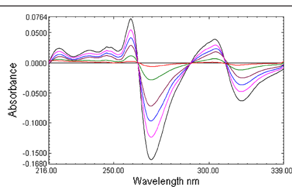
Figure 8 First derivative of the ratio spectra of CEF (1 to 15 µg/mL).
