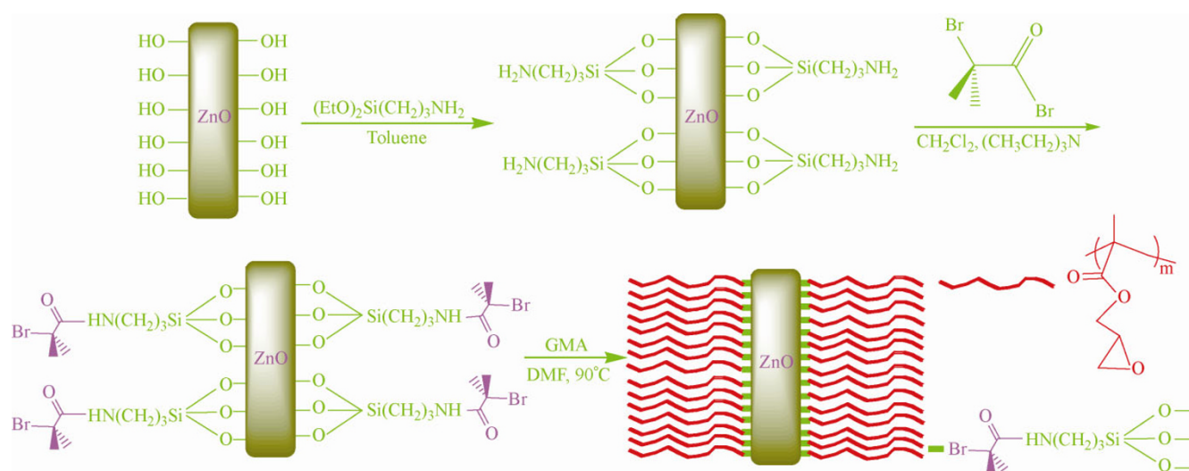
Scheme 1. Surface functionalization of ZnO Nanowires and polymerization of the initiator-functionalized wires.
