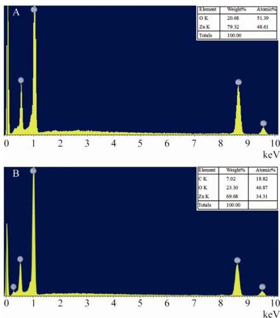
FIG. 2. Energy dispersive X-ray spectroscopy of (A) ZnO nanowires; (B) PGMA-ZnO nanowires.
