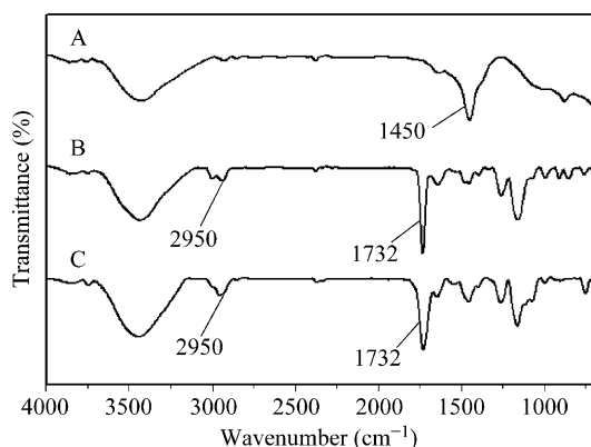
FIG. 3. IR spectra of (A) ZnO-NH 2 nanowires; (B) PGMA-ZnO nanowires; (C) after treatment of PGMA-ZnO nanowires in HCl solution.
