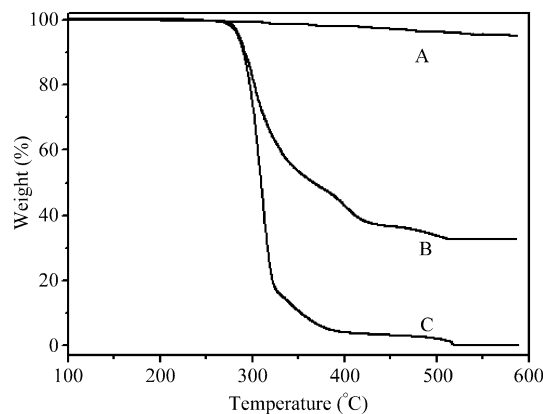
FIG. 4. TGA curve of (A) ZnO nanowires; (B) PGMA-ZnO nanowires; and (C) after PGMA-ZnO nanowires in HCl solution.
