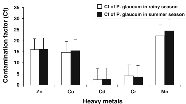
Fig. 9 Contamination factor of heavy metals in P. glaucum after irrigation with sugar mill effluent. Error bars are standard error of the mean
