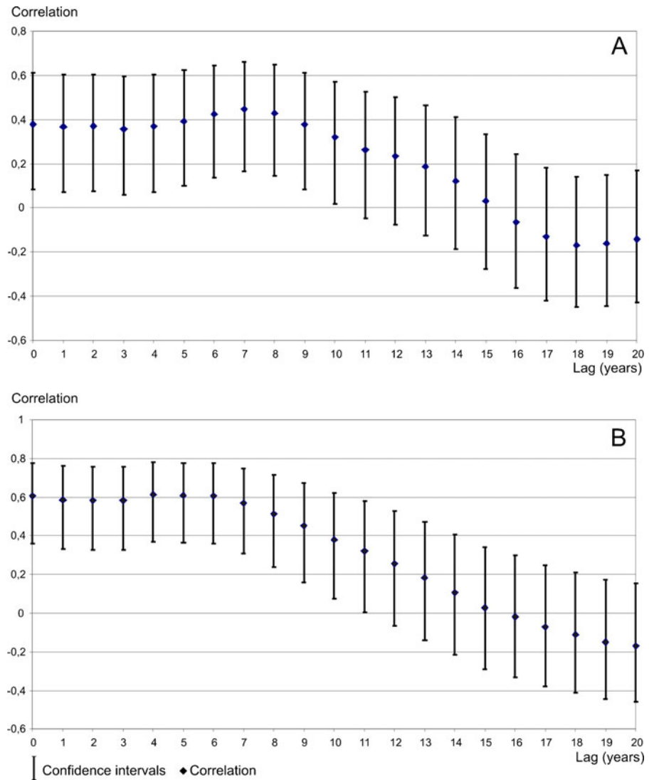
Fig. 11 Correlation and confidence intervals for total tree ring reductions, infant mortality rates and lung, bronchial, and tracheal cancer morbidity rates among males. a Results for lagged detrended infant mortality rates. b Results for lagged detrended lung, bronchial, and tracheal cancer morbidity rates among males
