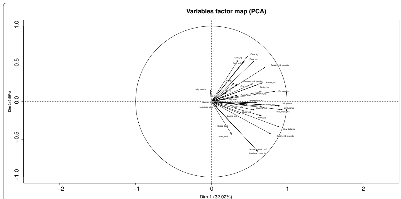
Fig. 6 PCA plot consisting of all the variables (35) measured in this study, showing their relative influence on the variation observed in the dataset, which is indicated as % on the first dimension (Dim 1) and the second dimension (Dim 2). This PCA also gives an indication of the grouping between all the variables measured. Variable labels: “Kcal_balance” = energy balance; “Fe_balance” = iron balance; “Zn_balance” = zinc balance; “Total_crops_m2” = total cropping area; “m2_person” = total cropping area per capita; “Tubers_m2_pcapita” = per capita area cultivated with tubers; “Cereals_m2_pcapita” = per capita area cultivated with cereals; “Legumes_m2_pcapita” = per capita area cultivated with legumes; “No_migrant” = number of household members migrating; “Mig_months” = number of months off-farm for migrating members. Livestock labels refer to total number of animals. Crop labels refer to total surface area in square meters (m 2 ) and total outputs in kilograms (kg). Arrow length is proportionate to the contribution made by an individual variable to the variation in the dataset. Directionality relative to other variables illustrates the nature of correlations (positive or negative) among variables. Crop outputs and per capita cropping areas (tubers, cereals, legumes) are shown to not only be largely driving variation in the data space ( long arrows ) but to also be positively correlated to energy, iron and zinc balances (same direction). The fact that livestock and household (size, migration) parameters are placed relatively far from the remaining variables further suggests that crop parameters have the strongest and most influential relations to household balance outcomes
