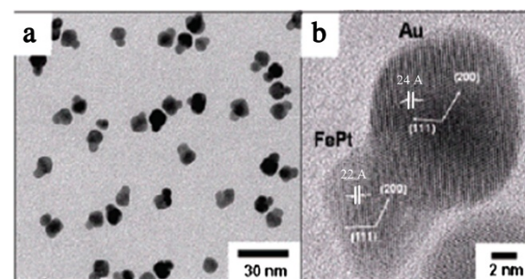
Figure 4 TEM and HRTEM images of FePt-Au heterostructured nanoparticles. (a) TEM image, and (b) HRTEM image of FePt-Au heterodimer nanoparticles reported by Choi et al. [50].
