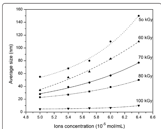
Figure 10 Exponential trend of changing average size of colloidal Al-Ni nanoparticles versus ion concentration for several doses [47].
