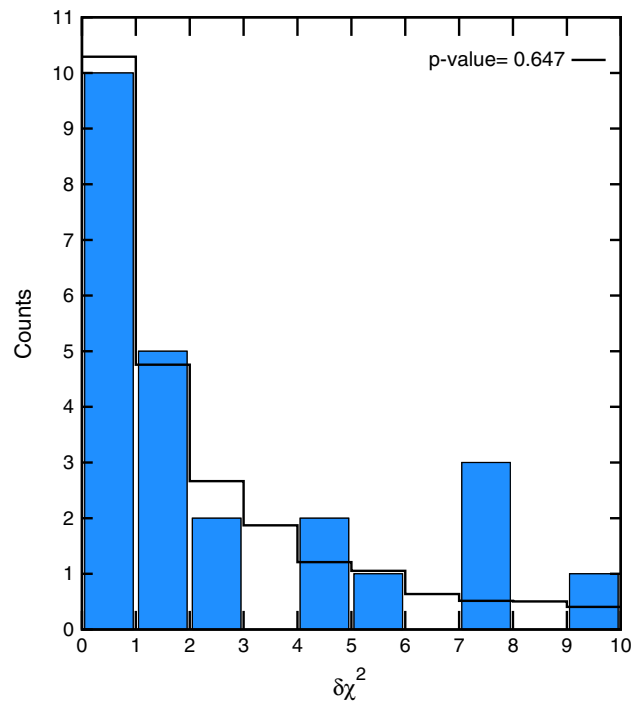
Fig. 2 The observed IceCube events (shaded histograms) and the simulated events (open histograms with continuous lines are for random RA) for different \delta\chi^2 distributions are shown for an angular resolution of the IceCube events \leq 40^\circ . The p values for the open histograms are also given
