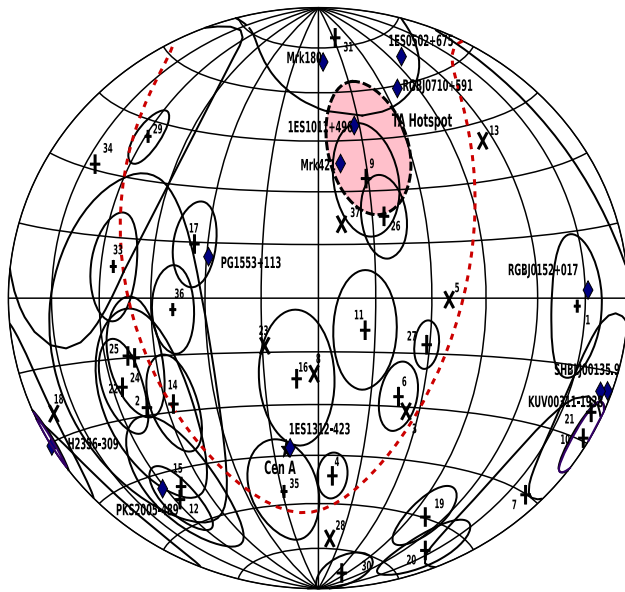
Fig. 1 The sky map is shown in the equatorial coordinates with the 37 IceCube events and their individual errors (only for shower events). Here plus signs are for are shower events and the times sign are for track events with their corresponding event ID. We have also shown the positions of the HBLs with their names, which are within the error circle of the IceCube events. The TA hotspot is shown as a shaded closed contour and the galactic plane is shown as a dashed line
