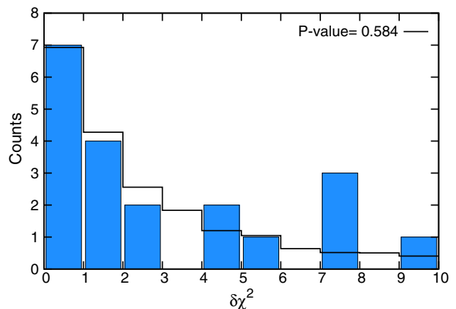
Fig. 3 Same as Fig. 2, but for an angular resolution of the IceCube events \leq 20^\circ
