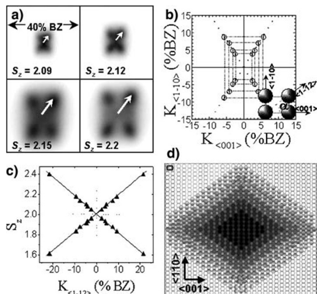
Fig. 4 Structural characterization of the RP state: (a) sequence of the (00) spot profile at several vertical scattering phases S_z (the arrows indicate the position of one satellite); (b) satellite position in the parallel momentum transfer plane K_{\langle -1-10 \rangle} - K_{\langle 001 \rangle} using S_z as a parameter; (c) plot of the satellite splitting as a function of S_z ; (d) simplified cartoon of a RP island with step edges running along well-defined \langle 1-12 \rangle directions. Darker colors correspond to topmost layers. The figure is reproduced from Ref. [17]
