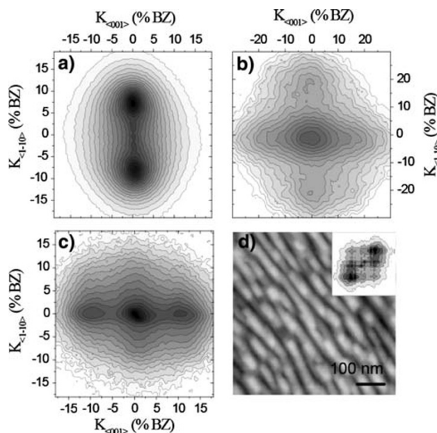
Fig. 2 Out-of-phase Spot Profile ( S_z = 2.2 ) after sputtering at: T = 450 K (a), T = 500 K (b), and T = 550 K (c). The axis scale is expressed in % of Brillouin Zone referred to the short side of the reciprocal surface cell. Panel (b) and (c) are reproduced from Ref. [17]. (d) AFM topography corresponding to an HTR morphology equivalent to panel (c) on a 600 \times 600 nm scale. Inset: FFT contour profile of the AFM image. \varepsilon = 1000 eV
