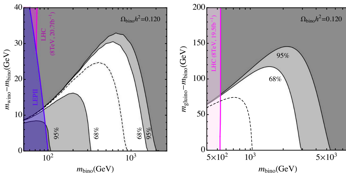
Figure 2. Left panel: the parameter region favored from the viewpoint of the dark matter relic abundance when the bino is the LSP and the wino is the NLSP. The light-gray and white regions are the same as those in figure 1. Limits from the LEP II and the LHC experiments at 95% C.L. are also shown. Right panel: the parameter region favored from the viewpoint of the dark matter relic abundance when the bino is the LSP and the gluino is the NLSP. The light-gray and white regions are the same as those in the left panel. A limit from the LHC experiment at 95% C.L. is also shown.
