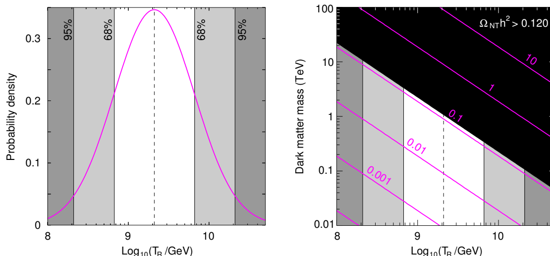
Figure 1. Left panel: the log-Gaussian probability density of T_R deduced from the BICEP2 result. The light-gray and white regions are the ones favored at 95% and 68% confidence level, respectively. See text for more details. Right panel: contours of \Omega_{\text{NT}} h^2 as a function of T_R and m_{\text{DM}} . The light-gray and white regions are the same as those in the left panel, while \Omega_{\text{NT}} h^2 exceeds the observed abundance in the black region.
