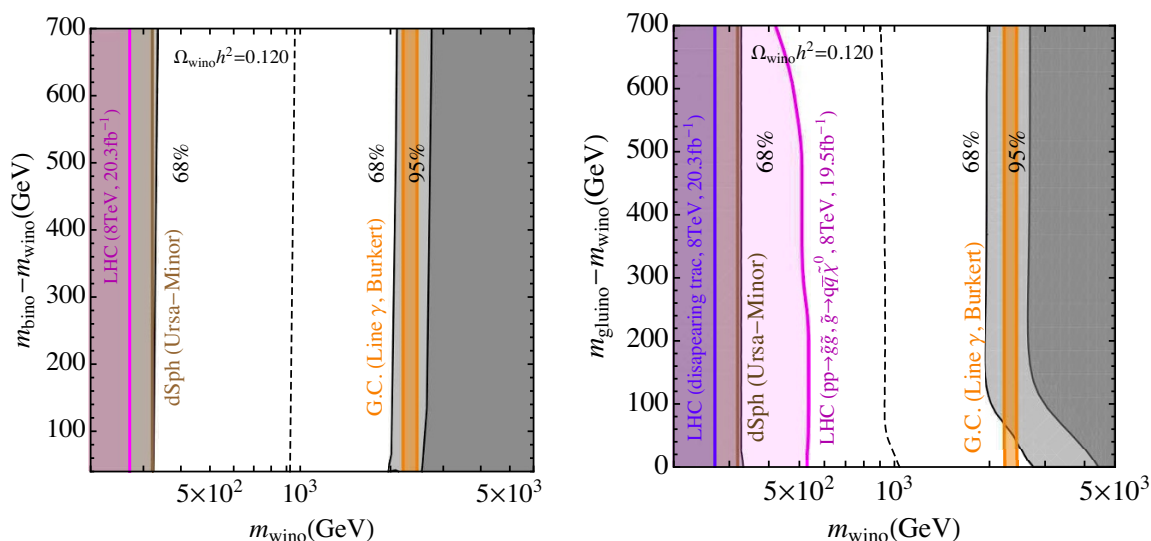
Figure 3. Left panel: the parameter region favored from the viewpoint of the dark matter relic abundance when the wino is the LSP and the bino is the NLSP. The light-gray and white regions are the same as previous figures. Limits from the LHC and the indirect dark matter detection (two kinds) experiments at 95% C.L. are also shown. Right panel: the parameter region favored from the viewpoint of the dark matter relic abundance when the bino is the LSP and the gluino is the NLSP. The light-gray and white regions are the same as those in the left panel. A limit from the LHC (two kinds) and the indirect dark matter detection (two kinds) experiments at 95% C.L. are also shown.
