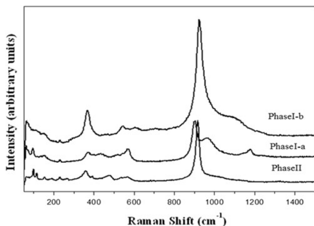
Fig. 9 Raman spectra of Cu-KDP (5) material in phase II, phase I-a and phase I-b
