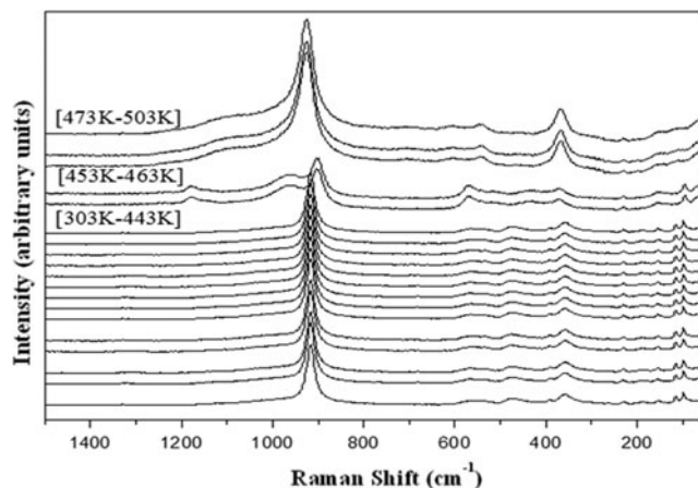
Fig. 8 Raman spectra of Cu-KDP (5) single crystal in the temperature range 303–503 K
