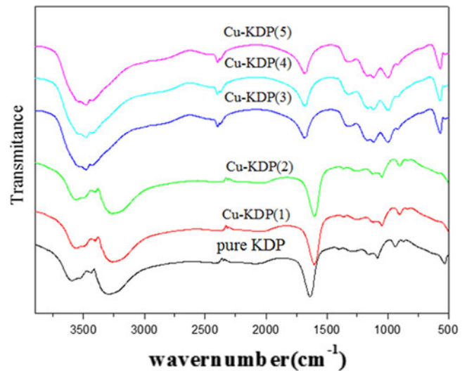
Fig. 5 FT-IR spectra recorded for the pure KDP, Cu-KDP (1), Cu-KDP (2), Cu-KDP (3), Cu-KDP (4) and Cu-KDP (5) at room temperature
