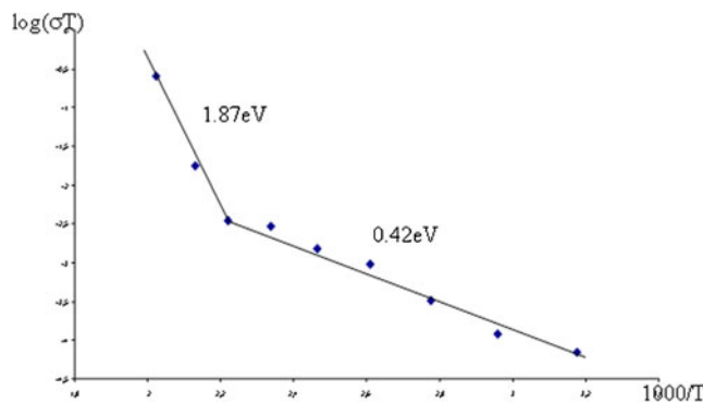
Fig. 12 Conductivity plots \log(\sigma T)=f(1,000/T) for Cu-KDP (5) compound
