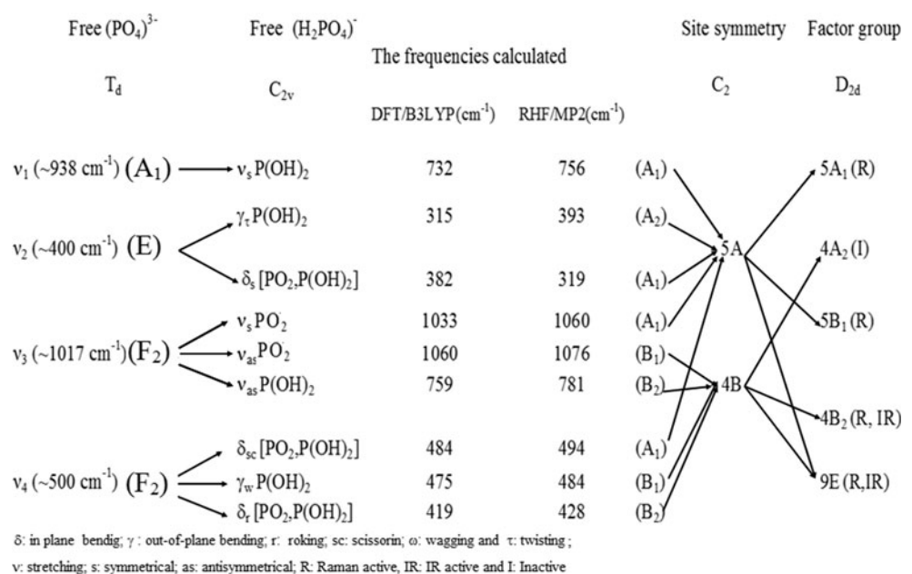
Fig. 6 Correlation scheme of internal vibration of the (\text{H}_2\text{PO}_4)^- in tetragonal Cu-KDP
