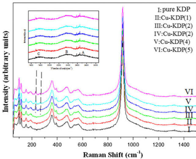
Fig. 4 Raman spectra for the pure KDP, Cu-KDP (1), Cu-KDP (2), Cu-KDP (3), Cu-KDP (4) and Cu-KDP (5) at room temperature
