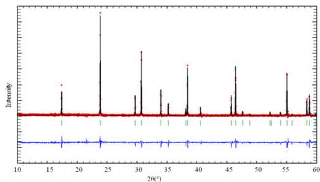
Fig. 2 The Pawley refinement of the lattice parameters of Cu-KDP (5). The point symbols represent the observed diffraction pattern, the solid lines represent the calculated pattern and the curves at the bottom of the figure represent the difference between the observed and calculated patterns. The short vertical lines mark the positions of possible Bragg reflections
