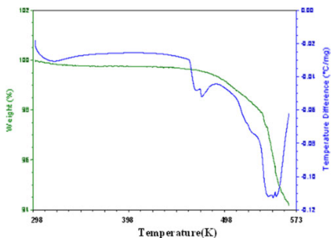
Fig. 3 Thermograms of DSC and TGA for Cu-KDP in the room temperature –573 K range
