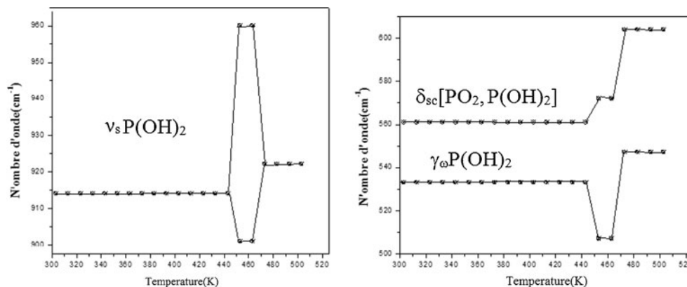
Fig. 10 The temperature dependence of the wavenumbers of some bands observed in the Raman spectra of the Cu-KDP (5)
