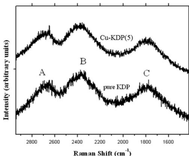
Fig. 7 ABC-type bands in the Raman spectrum for the pure and Cu-KDP (5) at room temperature
