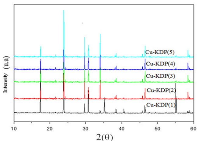
Fig. 1 The XRD patterns of Cu-KDP (1), Cu-KDP (2), Cu-KDP (3), Cu-KDP (4) and Cu-KDP (5)
