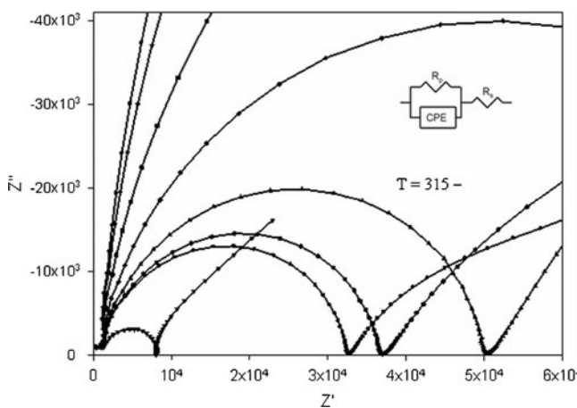
Fig. 11 Complex plane plots of Cu-KDP (5) at various temperatures
