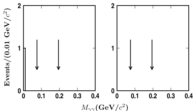
Fig. 2 Distributions of the \gamma\gamma invariant masses for the selected combinations of e^+e^- \rightarrow p\bar{p}K^+K^-\gamma\gamma from the \psi(3770) data ( left ) and the continuum data ( right ), where the pair of arrows denotes the \pi^0 signal region
