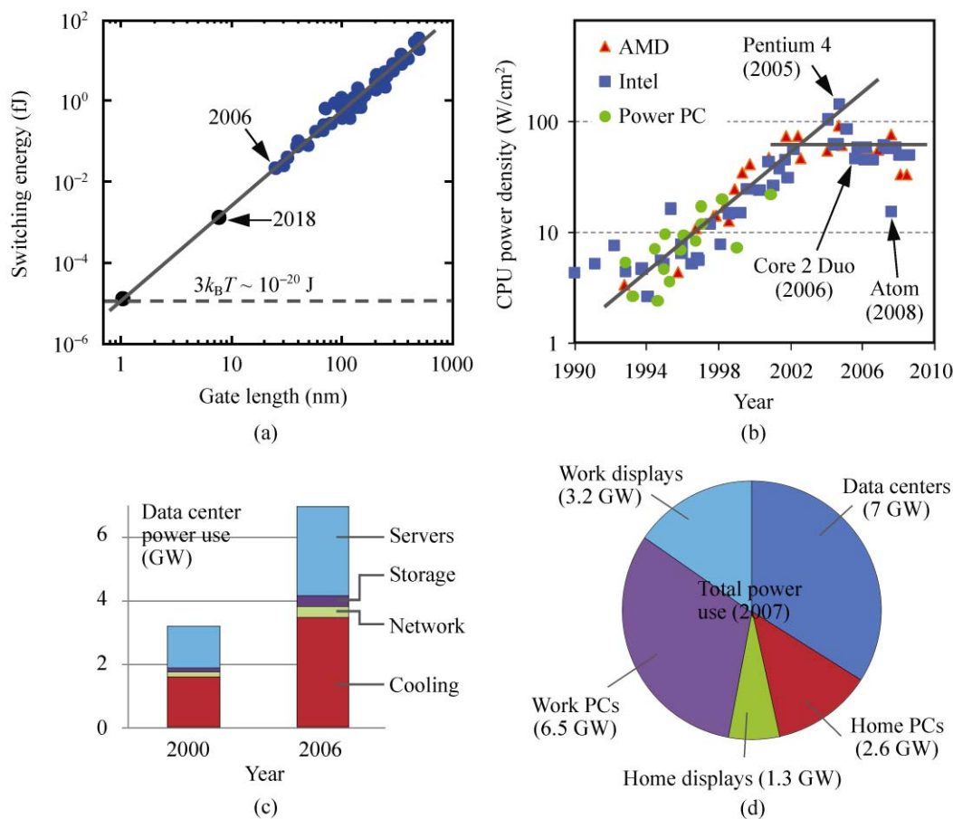
Figure 1 Energy and power dissipation from transistors, to CPUs, to data centers. (a) Switching energy of modern silicon transistors is still over 1000\times higher than fundamental physical limits, but on a trend toward them [3]. (b) Near-exponential increase of CPU power density in recent decades has flattened with the introduction of multi-core CPUs (solid lines show approximate trends); by comparison, the power density on the surface of the sun is approximately 6000 \text{ W}/\text{cm}^2 [2]. (c) Data center power use in the U. S. doubled in six years, with an extremely large proportion devoted to cooling. (d) Approximate breakdown of total power used by digital electronics in the U. S., where data are available [1, 6, 8]
