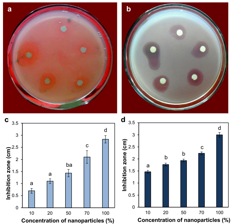
Figure 4 Antimicrobial effect of silver nanoparticles against normal and multidrug-resistant human bacteria E. coli by disc diffusion method. (a) Plate showing increasing inhibition zone of E. coli (DH5α) with increasing concentration of nanoparticles: clockwise from top 0.51, 1.02, 2.55, 3.57, and 5.1 μg in a total volume 100 μl in water. (b) Plate showing increasing inhibition zone of MDR E. coli (DH5α-MDR) with increasing concentration of nanoparticles: clockwise from top 0.51, 1.02, 2.55, 3.57, and 5.1 μg in a total volume 100 μl in water. (c) Graph of antimicrobial assay of the nanoparticles on E. coli (DH5α) in which 10, 20, 50, 70, and 100% nanoparticle solution corresponds to 0.51, 1.02, 2.55, 3.57, and 5.1 μg of silver nanoparticles in 100 μl solution, respectively. (d) Graph of antimicrobial assay of the silver nanoparticles on MDR E. coli (DH5α-MDR). Vertical bars indicate mean of three experiments ± standard error of mean (SEM). Different letters on bars indicate significant differences among treatments ( P=0.05 ).
