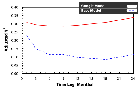
Figure 3 Effect of different delays in data availability on model quality. As the delay in availability of data on suicide occurrences varies for the public and policymakers, we perform the analysis for a range of possible delays. Specifically, we re-estimate the Google model in Eq. (3) using lags of 1, 3, 6, 9, 12, and 18 months, in addition to the original reporting delay of 24 months (x-axis). This covers delays in data availability for public (24 months delay), policymakers (around 6 months delay) and hypothetical models (a delay below 6 months). The adjusted R^2 values for the base model (dashed blue line) and the Google model (solid red line) with corresponding delays are shown on the y-axis. We observe that the results do not vary greatly when the lag in data availability is modified. The only mild deviation is observed for hypothetical delays of one or three months, where the base model improves, but in these cases too, the Google model still performs better than the base model. This provides further evidence of the potential value of online data in estimating suicide occurrence statistics.
