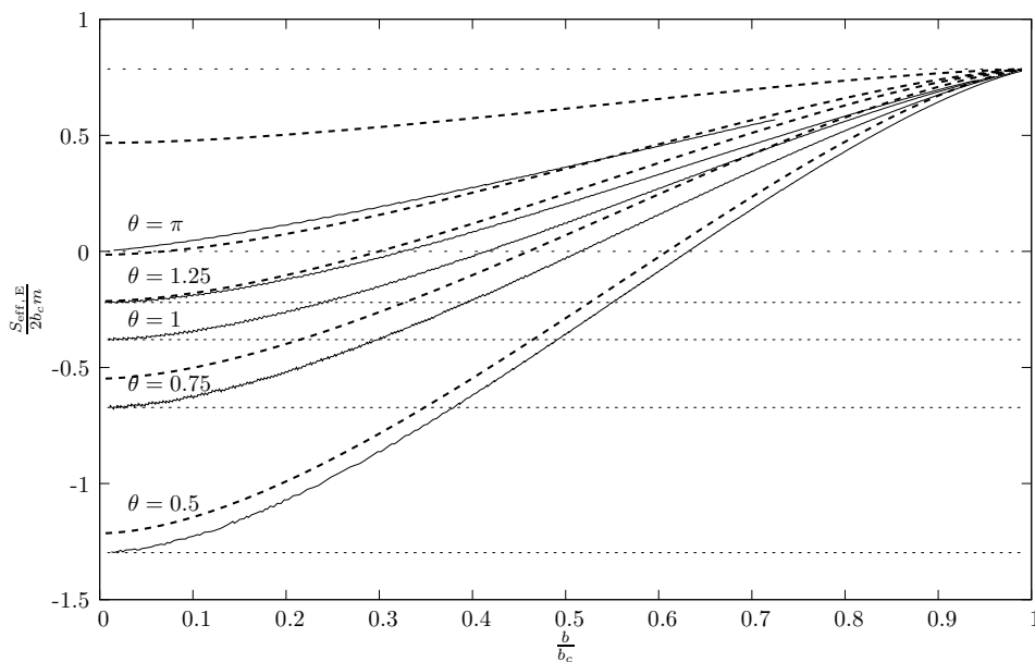
Figure 11. Effective action as a function of b for various values of \theta : “large” \theta . The key is as in figure 8. The values 0 and \pi/4 are plotted for reference with a dotted line with sparse dots.
