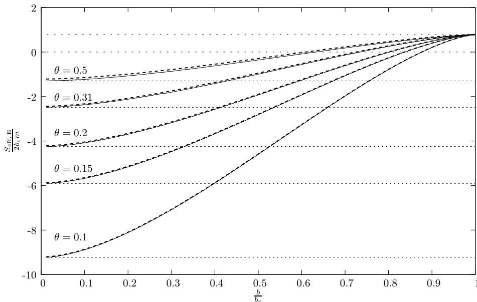
Figure 10. Effective action as a function of b for various values of \theta : small \theta . The action is plotted in units of 2b_c m = 8\pi\alpha'_{\text{eff}} m^2 . The key is as in figure 8. The values 0 and \pi/4 are plotted for reference with a dotted line with sparse dots.
