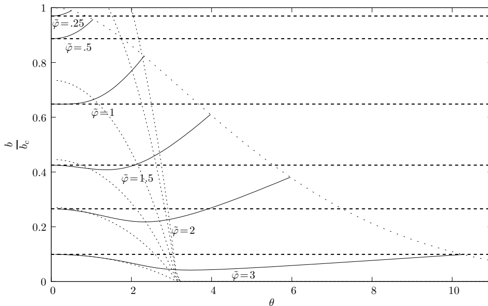
Figure 9. Curves of constant \tilde{\varphi} in the \theta - b plane. The key is as in figure 8. The dotted line with sparse dots corresponds to the limiting case \varphi_0 = 0 , i.e., \tau(0) = 0 , and is plotted for reference.
