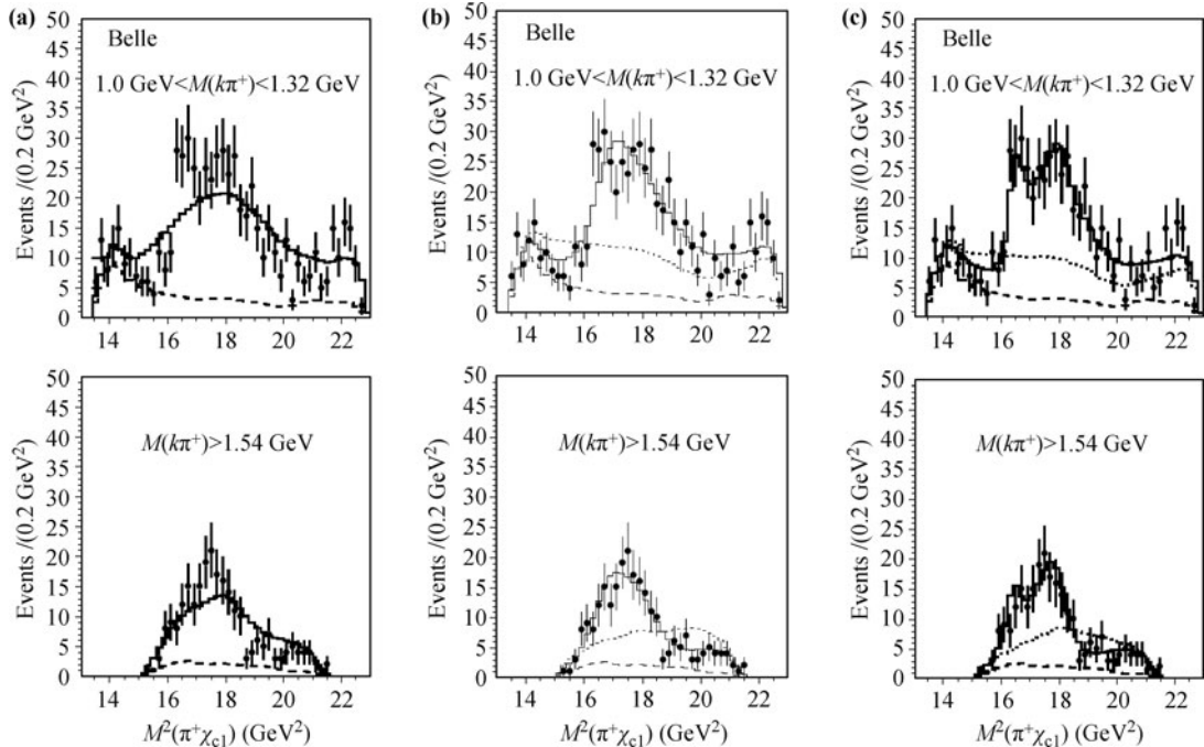
Fig. 9 (a) The M^2(\pi^+\chi_{c1}) distribution for B \rightarrow K\pi^+\chi_{c1} events with 1.0 \text{ GeV} < M(K\pi^+) < 1.32 \text{ GeV} ( upper ) and M(K\pi^+) > 1.54 \text{ GeV} ( lower ) from Belle. The solid histograms are projections of the two-dimensional fit with no resonance in the \pi^+\chi_{c1} channel. The dashed histogram indicates the background level determined from the \chi_{c1} mass sidebands. (b) The same data with results of the fit with a single Z^+ \rightarrow \pi^+\chi_{c1} resonance amplitude. Here the dotted histogram indicates the sum of all fit components other than the Z^+ . (c) The same data with results of the fit that includes two Z^+ \rightarrow \pi^+\chi_{c1} resonances with mass and width values given in the text.
