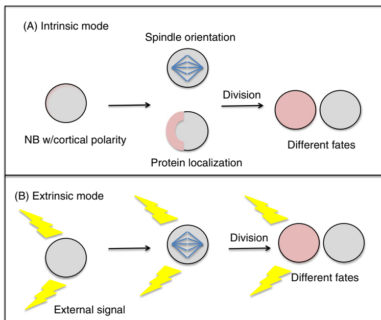
Figure 1 Intrinsic vs. extrinsic modes of asymmetric cell division. (A). During the intrinsic mode of asymmetric division, cells such as Drosophila neuroblasts possess an inherent axis of polarity. This polarity allows certain proteins such as cell fate determinants to localize asymmetrically within the cells. The mitotic spindle orients itself to be along the same axis of polarity, so when cellular division occurs, only one daughter cell receives the aforementioned determinants. Each daughter cell thus has a different fate. (B) During the extrinsic mode of asymmetric division, cellular precursors receive external, or extracellular, signals to self-renew (yellow). The mitotic spindle is oriented perpendicular to these external signals. When cellular division occurs, only one of the daughter cells continues to receive these signals and the two cells therefore have different fates.
