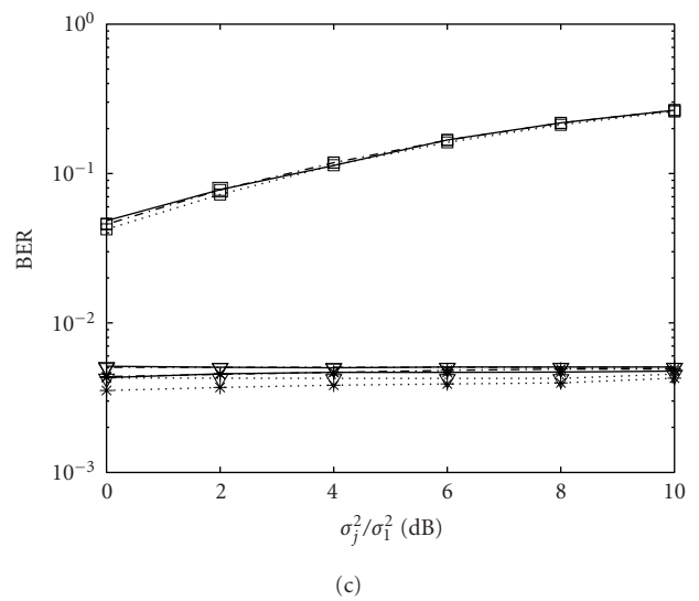
FIGURE 4: Near-far effect. (a) MSE. (b) Output SINR. (c) BER. The legend of (b) and (c) is the same as Figure 1b.
