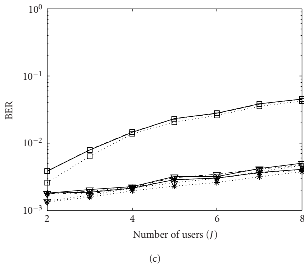
FIGURE 3: Effect of number of users. (a) MSE. (b) Output SINR. (c) BER. The legend of (b) and (c) is the same as Figure 1b.
