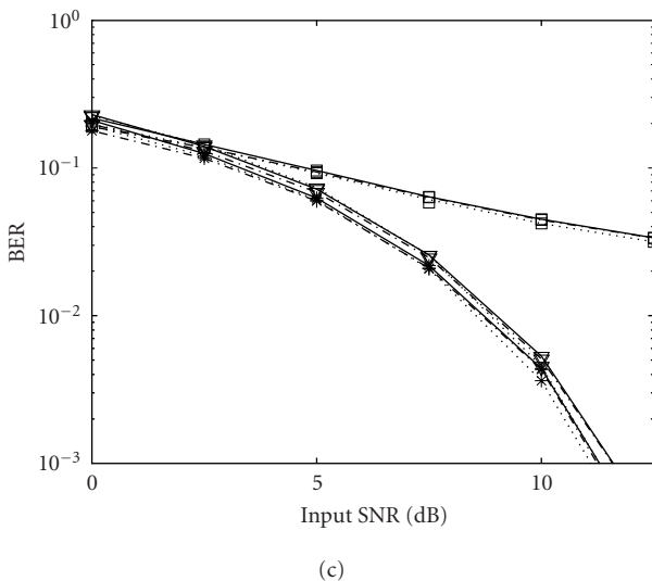
FIGURE 2: Effect of SNR. (a) MSE. (b) Output SINR. (c) BER. The legend of (b) and (c) is the same as Figure 1b.
