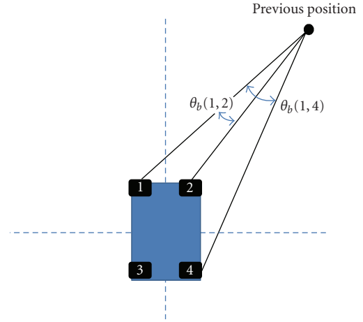
FIGURE 6: Minimizing GDOP per radio pair selection. The largest angle \theta_b(i, j) from the last position measurement indicates the smallest GDOP based on (4). This is used to determine which two radios are used for the next position measurement. In this case radio pairs (1, 4) yield the lowest GDOP.
