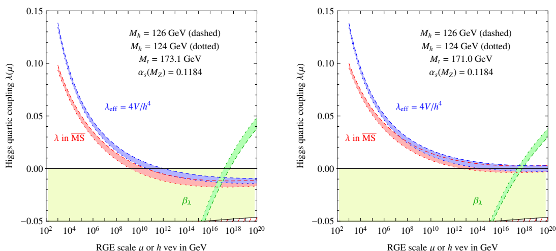
Figure 3. Evolution of the Higgs coupling \lambda(\mu) and its beta function, eq. (3.2), as a function of the renormalization scale, compared to the evolution of the effective coupling \lambda_{\text{eff}}(h) , defined in eq. (3.3), as a function of the field value. Left: curves plotted for the best-fit value of M_t . Right: curves plotted for the lower value of M_t that corresponds to \lambda(M_{\text{Pl}}) = 0 .
