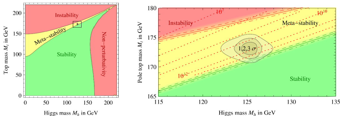
Figure 5. Regions of absolute stability, meta-stability and instability of the SM vacuum in the M_t - M_h plane. Right: zoom in the region of the preferred experimental range of M_h and M_t (the gray areas denote the allowed region at 1, 2, and 3\sigma ). The three boundaries lines correspond to \alpha_s(M_Z) = 0.1184 \pm 0.0007 , and the grading of the colors indicates the size of the theoretical error. The dotted contour-lines show the instability scale \Lambda in GeV assuming \alpha_s(M_Z) = 0.1184 .
