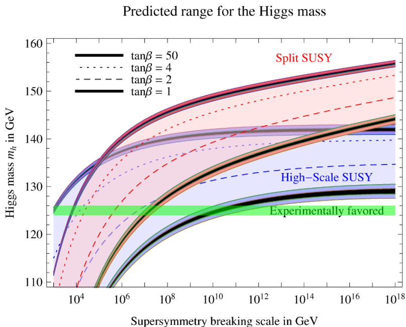
Figure 8. NNLO prediction for the Higgs mass M_h in High-Scale Supersymmetry (blue, lower) and Split Supersymmetry (red, upper) for \tan\beta = \{1, 2, 4, 50\} . The thickness of the lower boundary at \tan\beta = 1 and of the upper boundary at \tan\beta = 50 shows the uncertainty due to the present 1\sigma error on \alpha_s (black band) and on the top mass (larger colored band).
