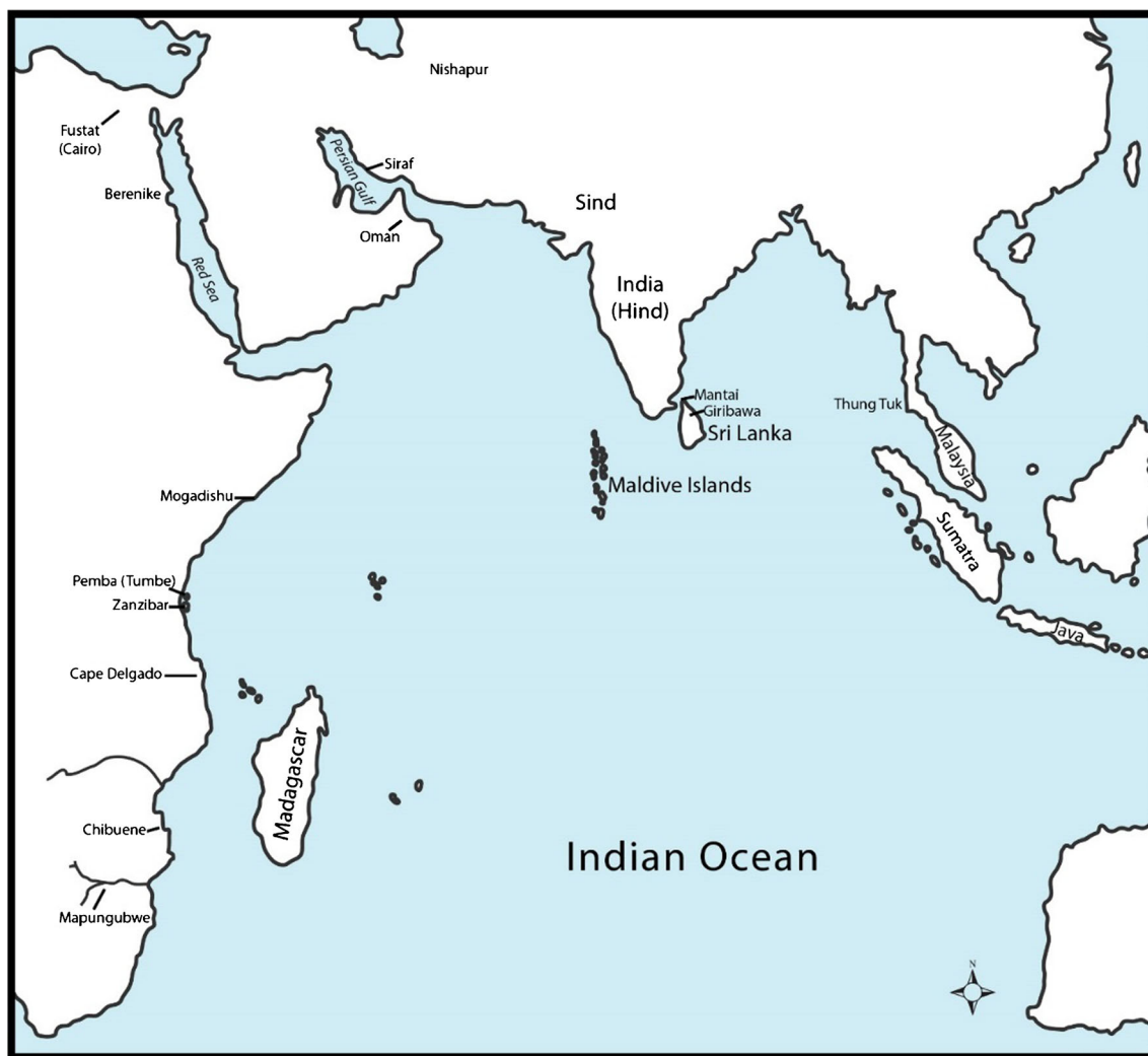
Fig. 1 Indian Ocean map with places mentioned in the text
