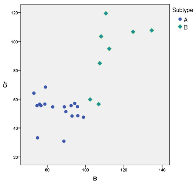
Fig. 6 Plot of chromium vs boron for the v-Na-Ca A and B samples. Measurements in parts per million
