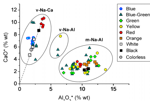
Fig. 3 Plot of lime vs alumina for all analyzed Zanzibar beads (reduced compositions calculated using the method of Panighello et al. (2012))
