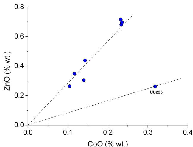
Fig. 7 Correlation between zinc and cobalt in the blue Zanzibar beads
