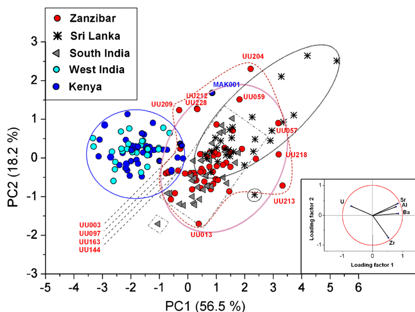
Fig. 4 PCA of m-Na-Al samples based on U, Ba, Zr, Sr, and Al levels. The Zanzibar beads are compared to others from Sri Lanka (Dussubieux 2001) and South India, West India, and Kenya (data courtesy of Dussubieux; see also Dussubieux et al. 2008, 2010). The black oval delineates samples from Sri Lanka, while the gray dashed-dotted rectangle outlines the South Indian ones. The red dashed line includes
