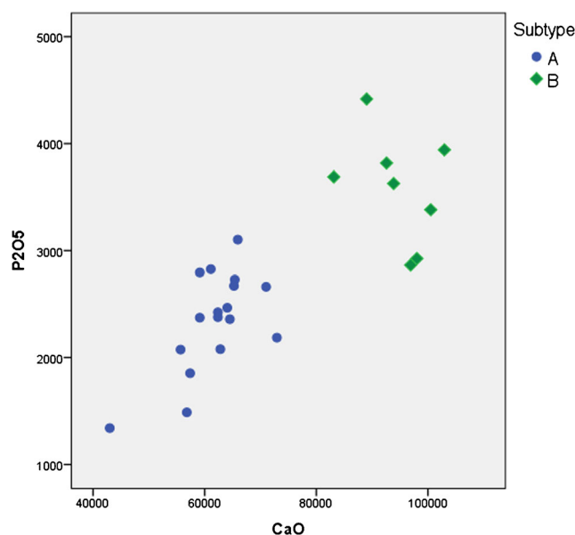
Fig. 5 Plot of lime vs phosphorus pentoxide for the v-Na-Ca A and B samples. Measurements in parts per million
