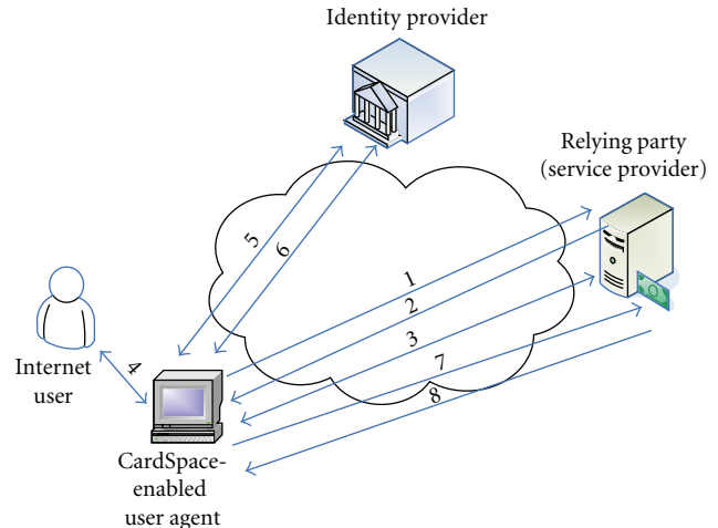
FIGURE 1: CardSpace framework.
