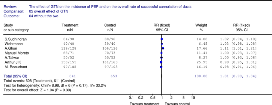
Figure 4 This figure revealed the overall effect of GTN on the successful rate of cannulation.
