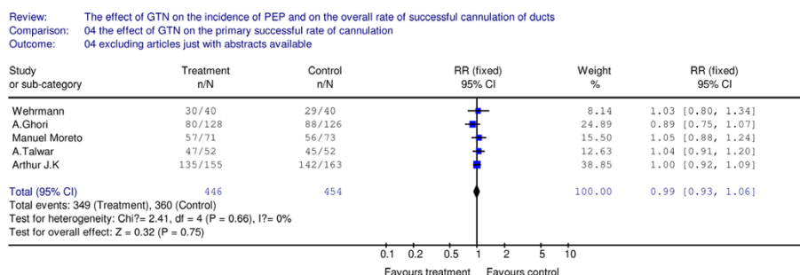
Figure 3 This figure revealed the primary effect of GTN on the successful rate of cannulation.
