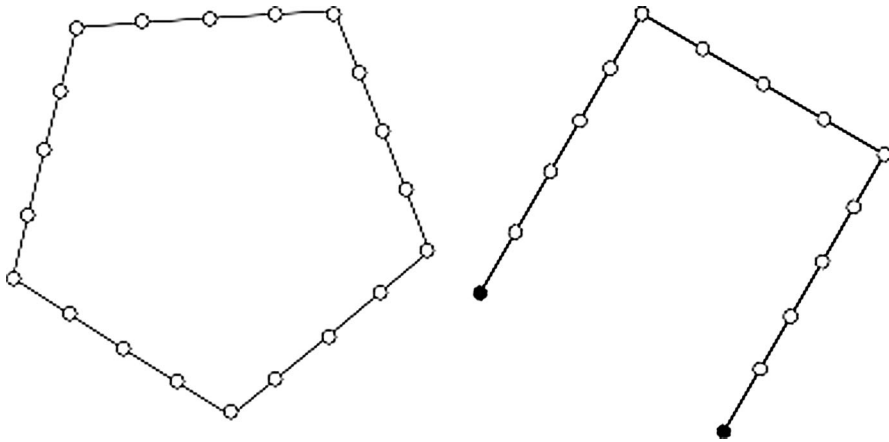
Fig. 1 Greechie diagrams of two OMLs which, if supplied with the state which assigns the number \frac{1}{5} to all “white” atoms and 0 to both “black” atoms, form non-classical probability spaces which are causally up-to-2-closed (or simply “causally closed”, to use the term of Gyenis and Rédei (2004) w.r.t. L_{ind}^+
