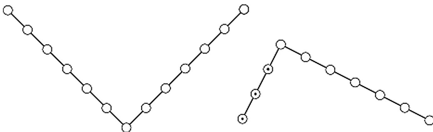
Fig. 2 In these OMLs “white” atoms have probability \frac{1}{7} and the “dotted” ones \frac{2}{7} . The space depicted on the left is causally up-to-3-closed, but the one on the right is not
