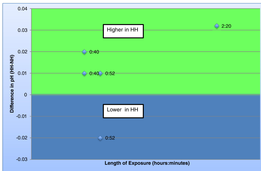
Figure 6 Graph of pHs. Graph to show the difference in pH between the two environments over time. Each data point represents data obtained from a study and the number refers to the time point. If the data point is in the green area, the pH was found to be higher in HH but if in the blue area, the pH was found to be lower in HH.
