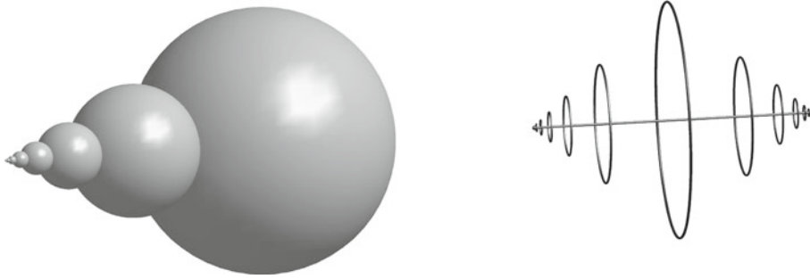
Figure 1: Left a union of countably many spheres is in \mathcal{F}(2) \cap \mathcal{A}(\delta) . Right a set in \mathcal{F}(1) \setminus \mathcal{A}(\delta)
