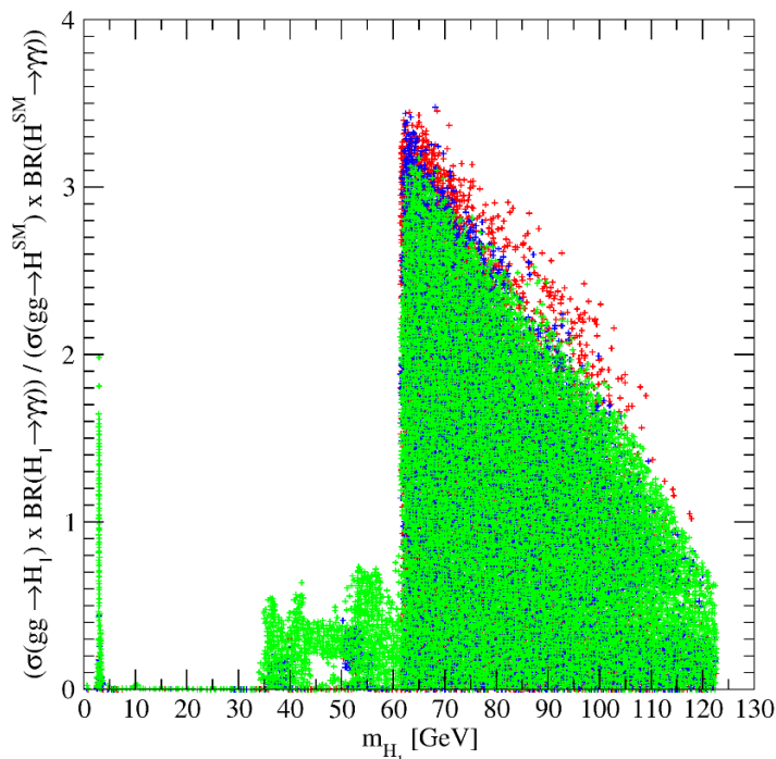
Figure 7. The H_1 signal rate in gluon fusion and the \gamma\gamma channel relative to a SM-like Higgs boson H^{SM} of the same mass. The color code is as in figure 1.
