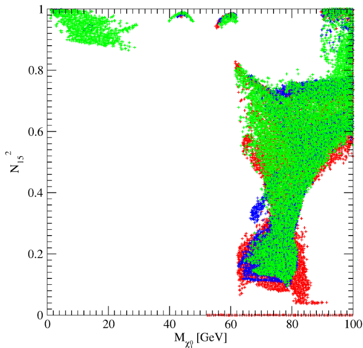
Figure 6. The \chi_1^0 singlino component (squared) as function of M_{\chi_1^0} . The colors are as in figure 1.
