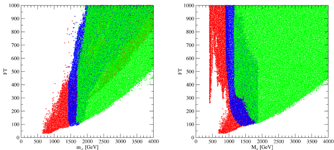
Figure 2. FT as defined in (2.10) as function of the squark and gluino masses, and the impact of the LHC constraints in the same color coding as in figure 1.
