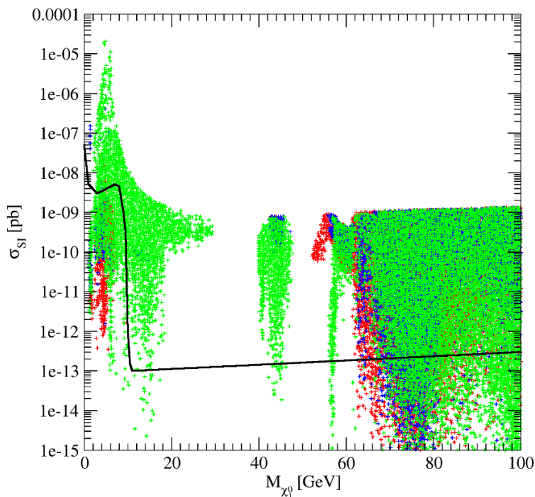
Figure 5. The spin-independent \chi_1^0 -nucleon cross section \sigma_{SI} (after imposing constraints from the LUX experiment [5]) as function of M_{\chi_1^0} , focussing on M_{\chi_1^0} < 100 GeV. The black line indicates the expected neutrino background to future direct dark matter detection experiments (from [70]). The colors are as in figure 1.
