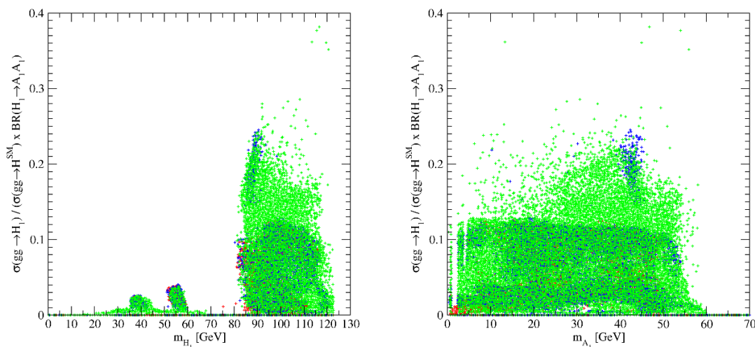
Figure 8. \sigma_{H_1}(ggF)/\sigma_{H^{SM}}(ggF) \times BR(H_1 \rightarrow A_1 A_1) as function of M_{H_1} (left) and M_{A_1} (right). The color coding is as in figure 1.
