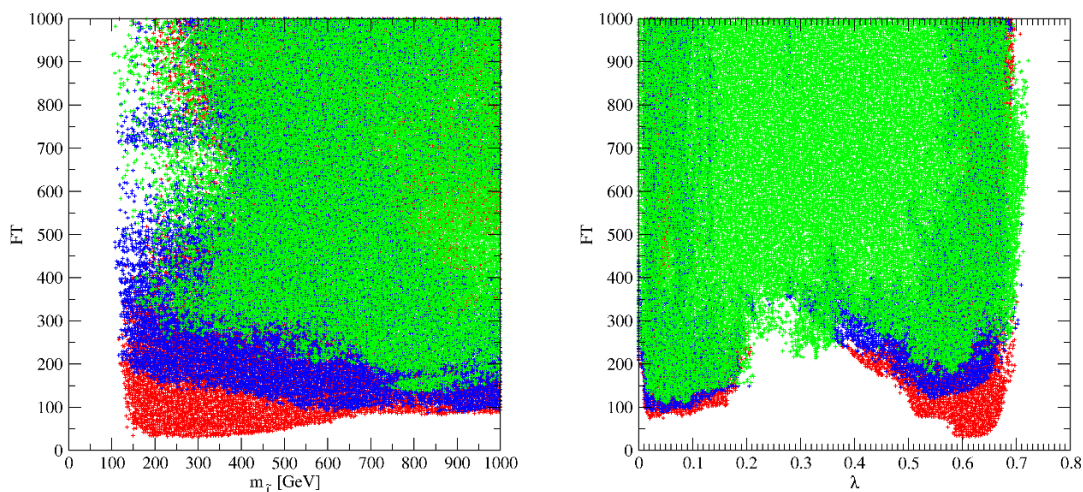
Figure 3. Left: FT as function of the m_{\tilde{t}_1} . Right: FT as function of \lambda at the SUSY scale. The color coding is as in figure 1.
