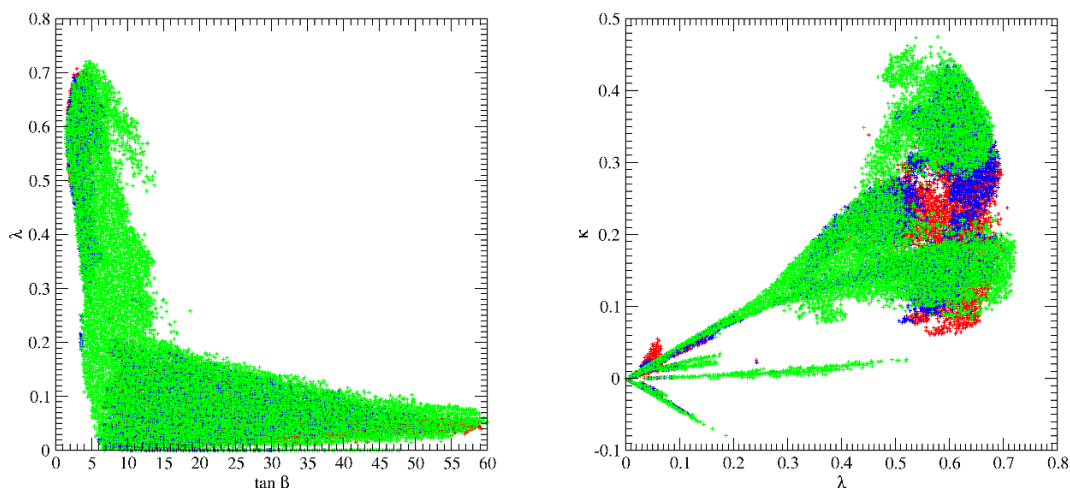
Figure 4. Left: \lambda as function of \tan\beta . Right: \kappa as function of \lambda . The colors are as in figure 1.
