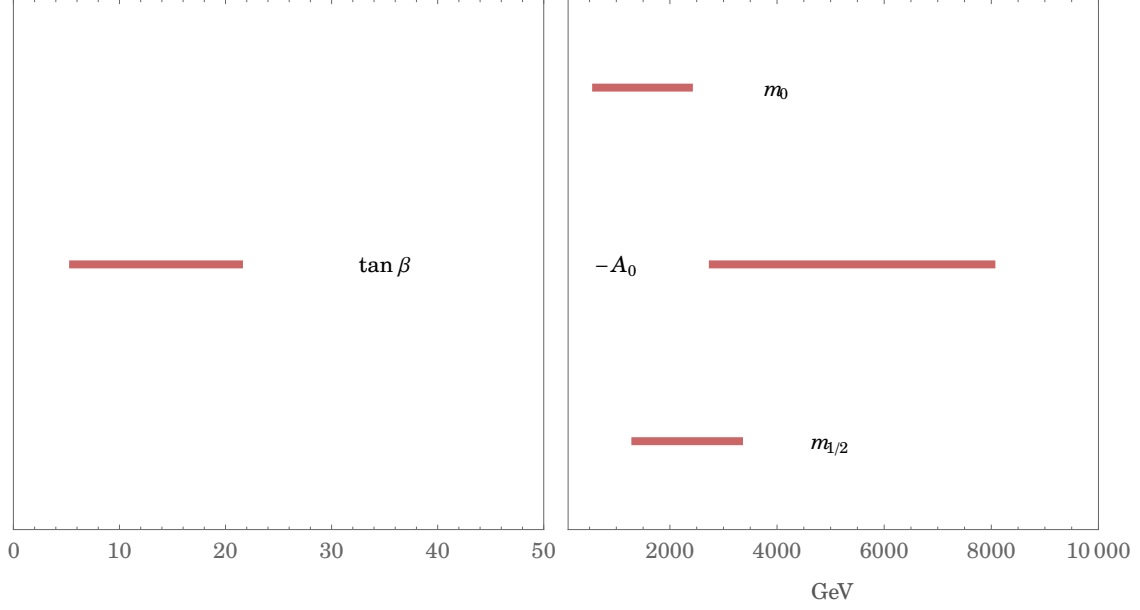
Figure 12. 1\sigma HPD intervals for the Constrained MSSM soft-breaking parameters.
