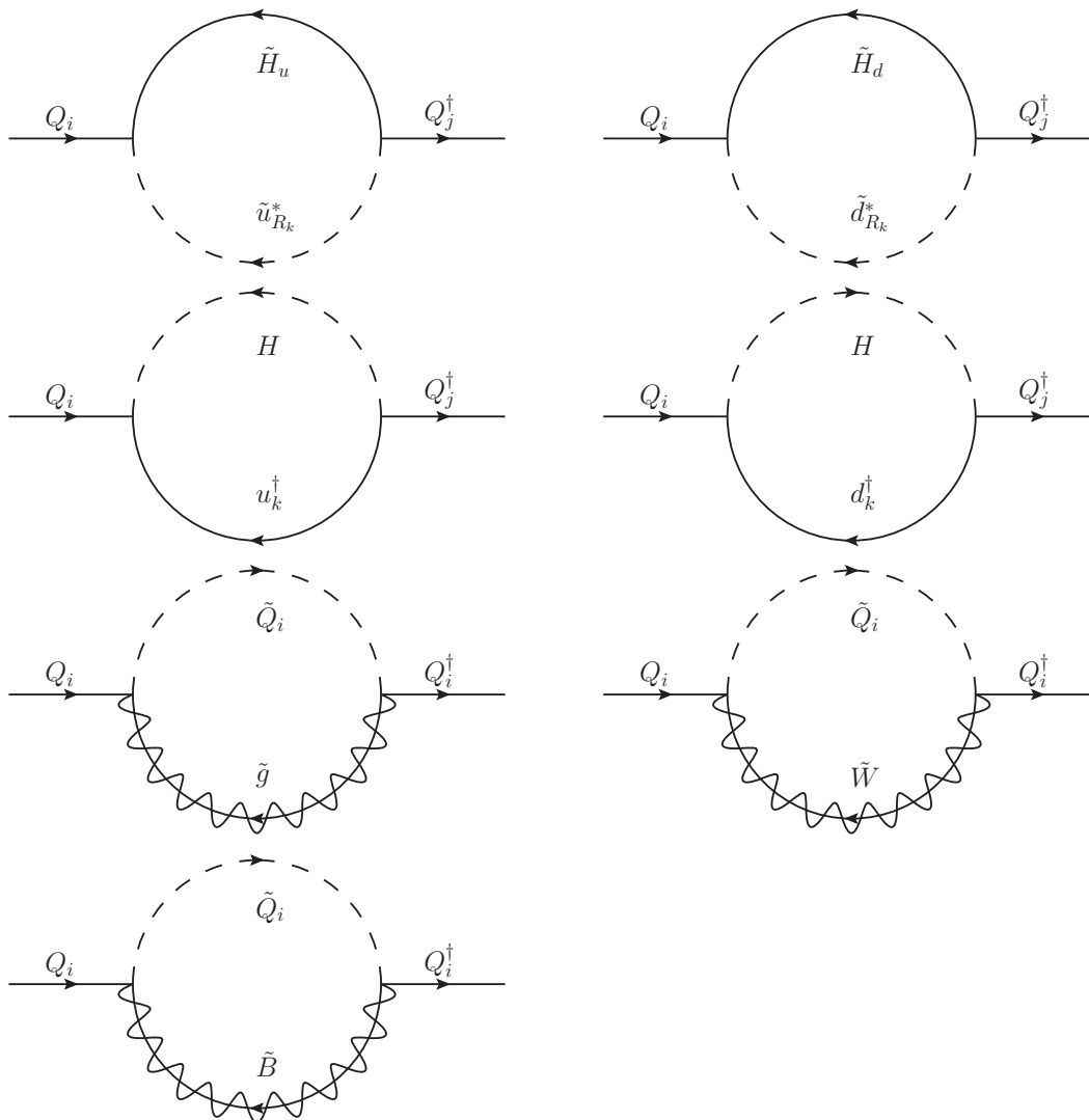
Figure 7. Loops contributing to threshold corrections from canonical normalization of external quark doublets.
