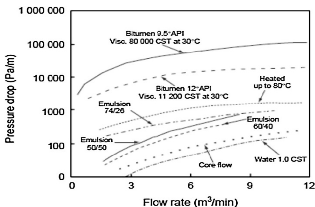
Fig. 2 Pressure drop against flow rate for the different heavy crude transport mechanisms Guevara et al. (1998)
