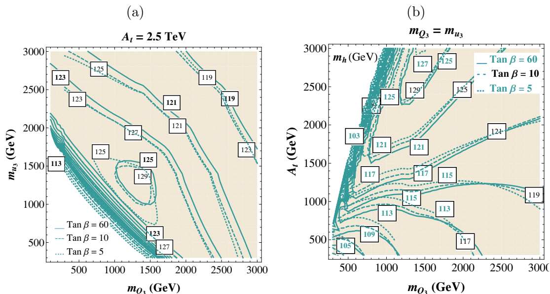
Figure 2. Contour plots of the Higgs mass in the plane of soft supersymmetry breaking parameters in the stop sector. In (a), we show the Higgs masses for A_t = 2.5 TeV for three different values of \tan\beta , \tan\beta = 5 (dotted lines, green (grey) labels), \tan\beta = 10 (dashed lines, black labels) and \tan\beta = 60 (solid lines, green (grey) labels). The masses for \tan\beta = 60 shown are smaller than the ones for \tan\beta = 10 mostly due to the negative effects from the staus (see eq. 2.6), and closer to the \tan\beta = 5 ones. In (b), the Higgs mass contours are shown for m_{Q_3} = m_{u_3} , varying the stop mixing parameter A_t . The stau supersymmetry breaking parameters have been kept at m_{L_3}^2 = m_{e_3}^2 = (350\text{GeV})^2 and A_\tau = 500 GeV, while \mu = 1030 GeV.
