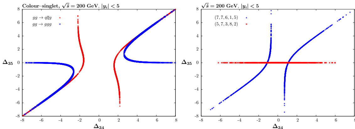
Figure 1. Scan of solutions to (3.16) and (3.27) which lie in the physical region. (Left) Solutions for the gg \rightarrow q\bar{q}g and gg \rightarrow ggg amplitudes for which the incoming gluons are in a colour-singlet state. For the quark amplitude, the case where the gluon and quark are aligned (with momenta defined as in (3.26)) is shown; if the gluon and anti-quark are aligned the corresponding curve is simply reflected around the line \Delta_{34} = \Delta_{35} . (Right) Solutions for the 5-gluon amplitudes, for two different colour choices (c_1, c_2, c_3, c_4, c_5) . The central system mass is \sqrt{\hat{s}} = 200 GeV, and the final-state particles are required to have rapidity |y_i| < 5 .
